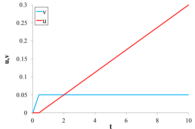
Figure 7: Loading history.
