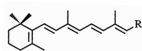
Formula I: Structure of the parent compound of retinoids
