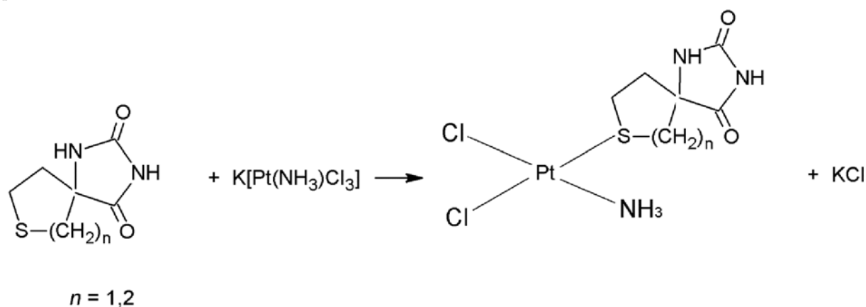
Fig. 1. General scheme of synthesis of new platinum complexes V and VI.
