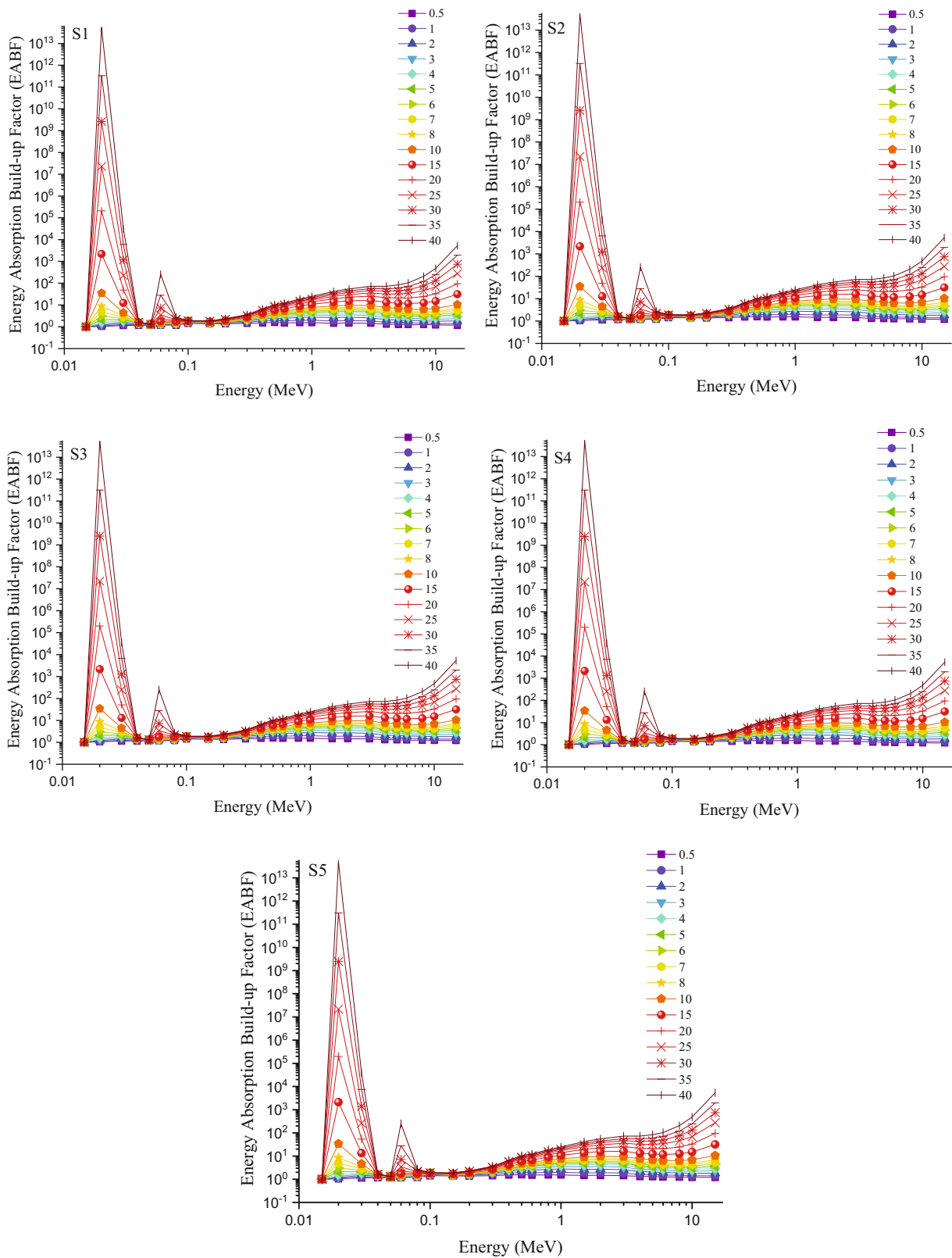
Figure 7: Variation of EABFs of investigated glasses at different MFP values.
