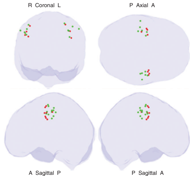
Figure 3: Dipole localizations for all subjects, obtained with the different co-registration procedures (red: based on three AL and green: IM). The IM based dipoles are located more lateral and posterior in most cases.
