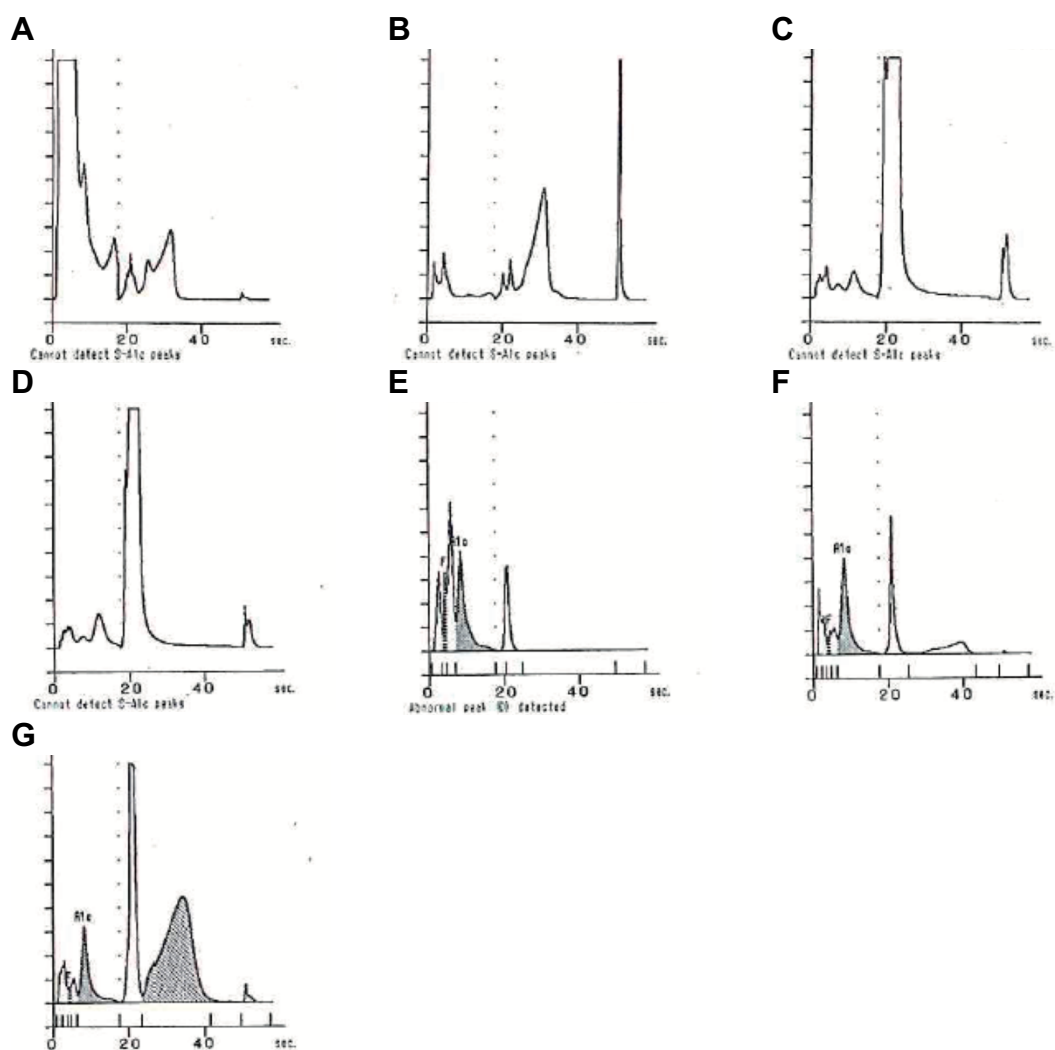
Supplementary Figure 4 – Homozygous Hb variants and uncommon Hb variants. Chromatograms of A. HbSS B. HbSC C. HbEE D. HbDD. E. HbAJ. F. HbAO-Arab G. HbAQ-Iran.
