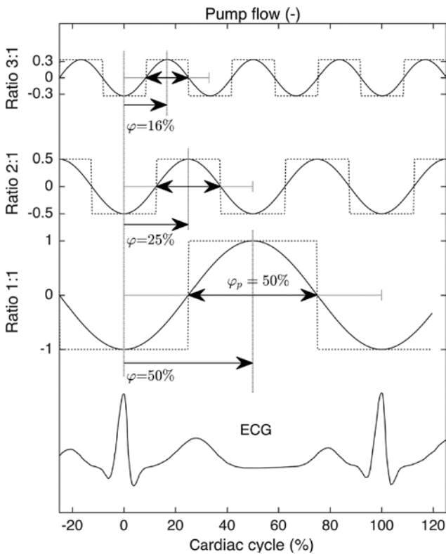
Figure 1: Definition of the phase shift ( \varphi ) and the systolic fraction ( \varphi_p ).
