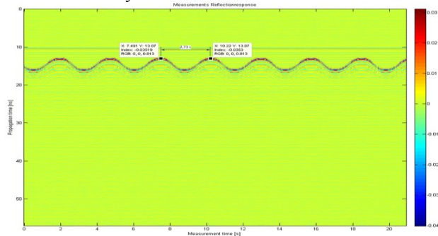
Figure 5: Radargram covering a generated motion
