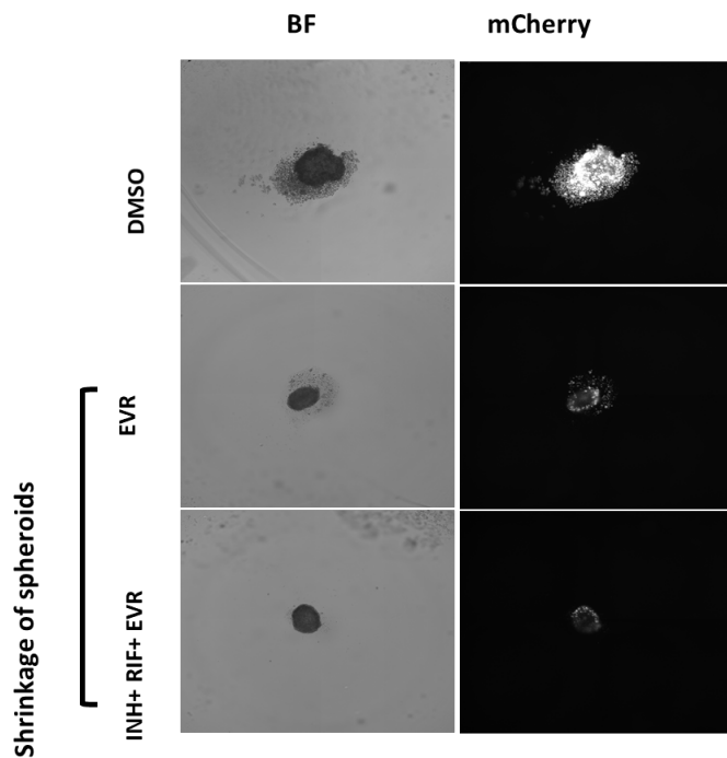
Supplementary Figure S1: Size of spheroids with Everolimus treatment. Representative images of spheroids treated with DMSO (0.5% v/v), EVR (1 nM) and a combination of INH, RIF and EVR (0.625 \mu M INH, 0.195 \mu M RIF and 1 nM EVR).
