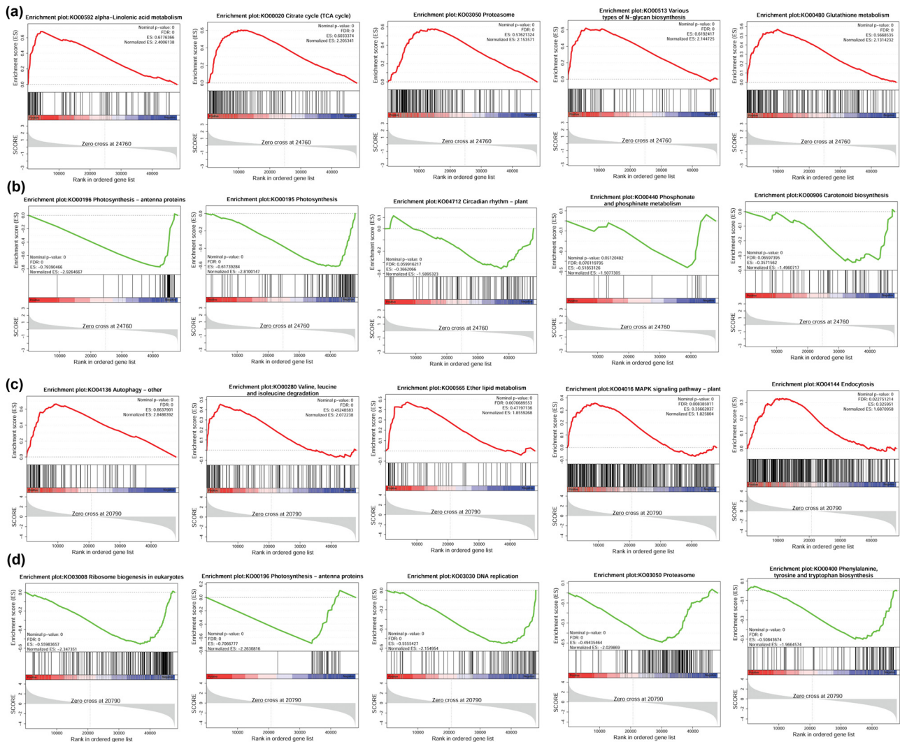
Figure S2: Results of GSEA based on KEGG. (a) and (b) Top 5 positively and negatively correlated pathways for DEGs in LT-CK vs LT. (c) and (d) Top 5 positively and negatively correlated pathways for DEGs in HT vs LT.
