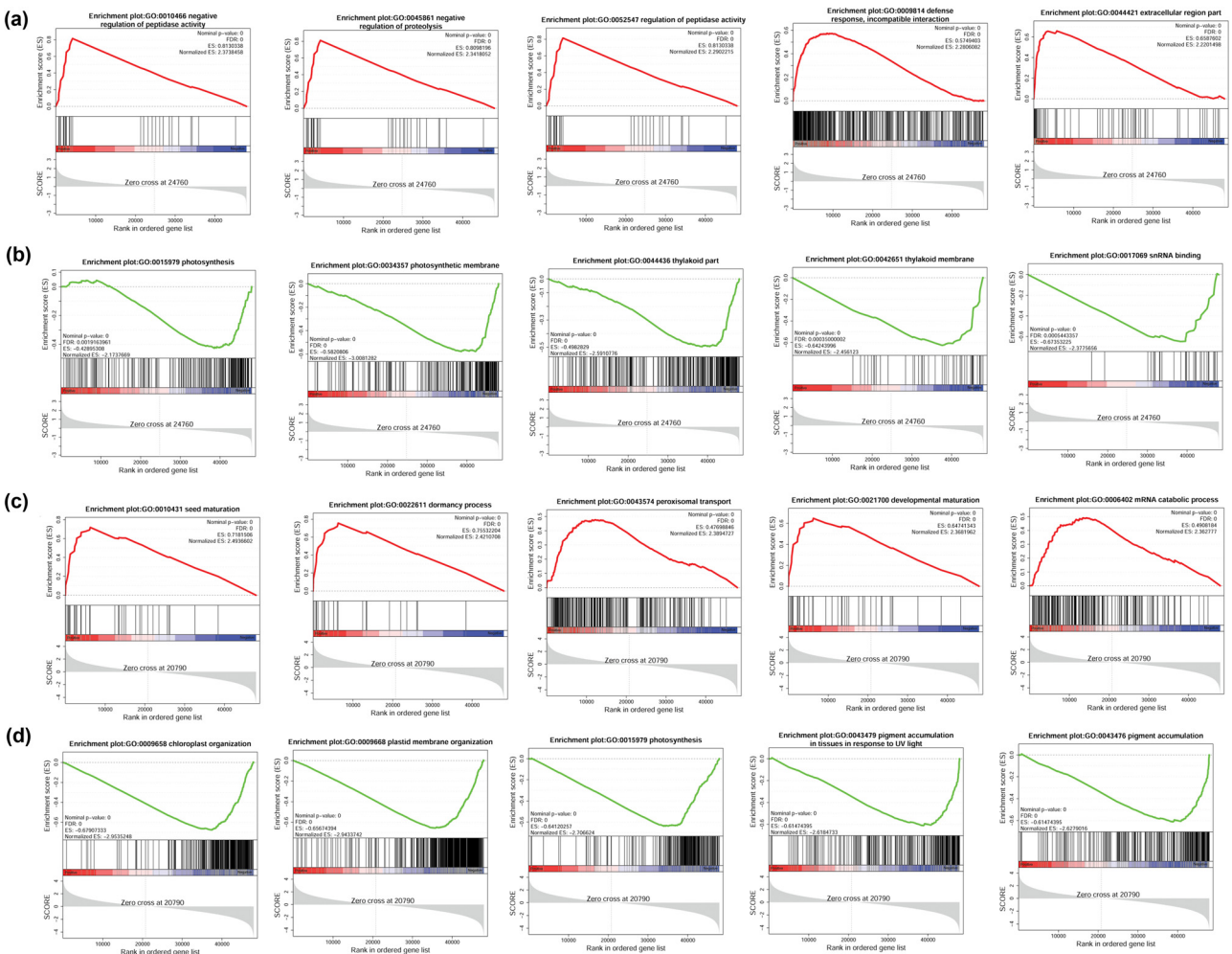
Figure S1: Results of GSEA based on GO. (a) and (b) Top 5 positively and negatively correlated GO terms for DEGs in LT-CK vs LT. (c) and (d) Top 5 positively and negatively correlated GO terms for DEGs in HT vs LT.
