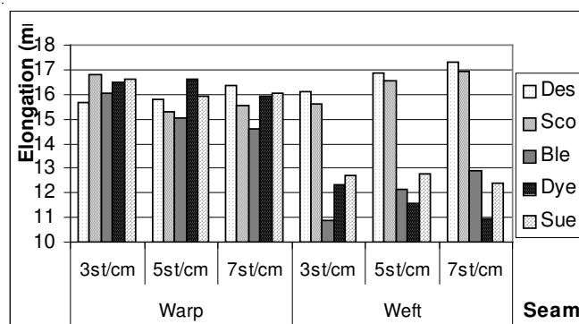
Figure 9. Elongation at break for different density for all treatment.
