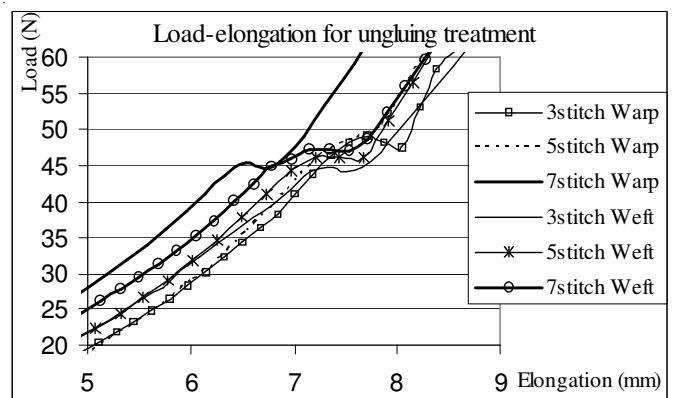
Figure 13. Load-elongation for ungluing treatment
