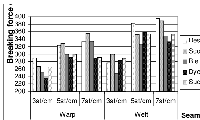
Figure 8. Breaking force for different density for all treatment.
