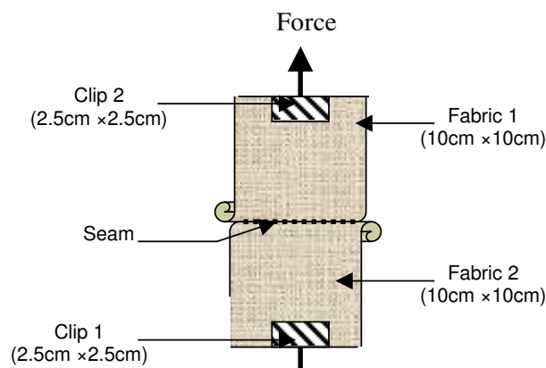
Figure 3. Seamed fabric under load.
