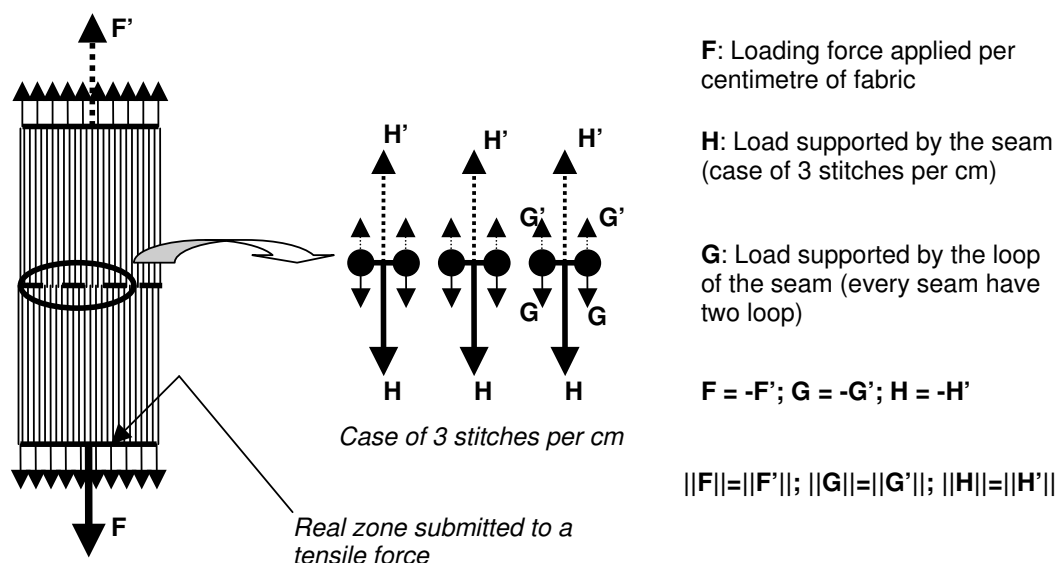
Figure 6. Load sharing to the seam.
