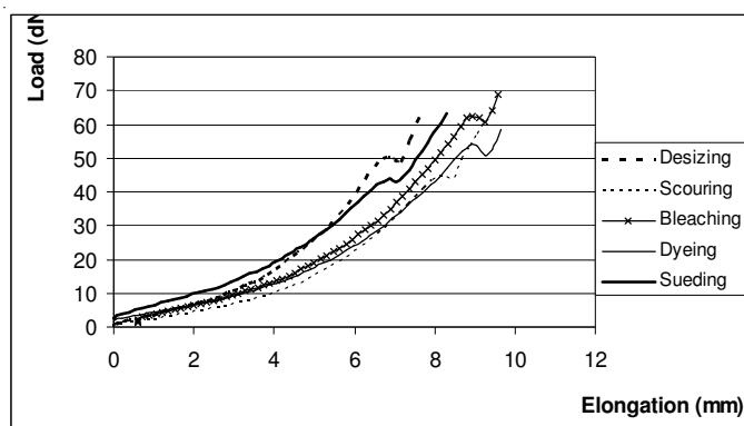
Figure 11. Load-elongation for seam in warp direction.
