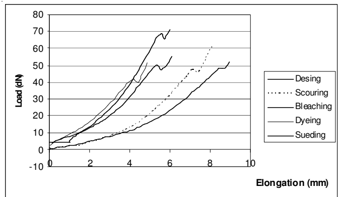
Figure 12. Load-elongation for seam in weft direction.
