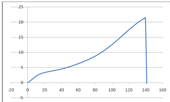
Figure 4. Strength[N]/elongation[mm] curve of sewing yarn before sewing.
