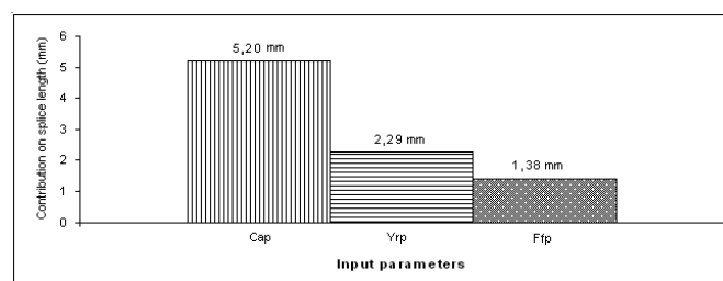
Figure 7. The increase of splice length as function of increase of Schlafhorst splicer parameters levels.
