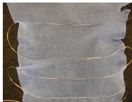
Figure 12. Optical fibre of 0, 75 mm integrated in rectangular piece.
