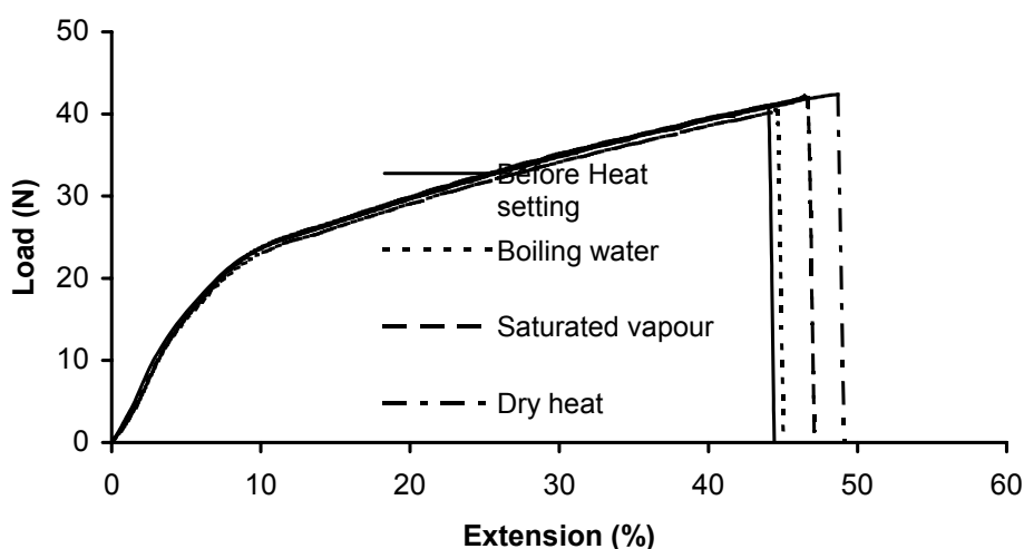
Figure 3. Load-extension curves of braided suture
