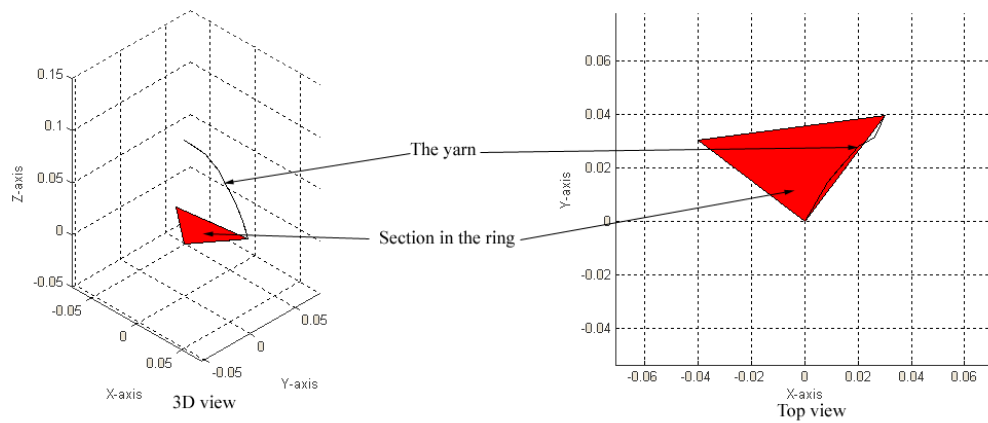
Figure 8a. Yarn balloon in a transitional state – 3D and top view (at 1.5 ms after starting simulation)
