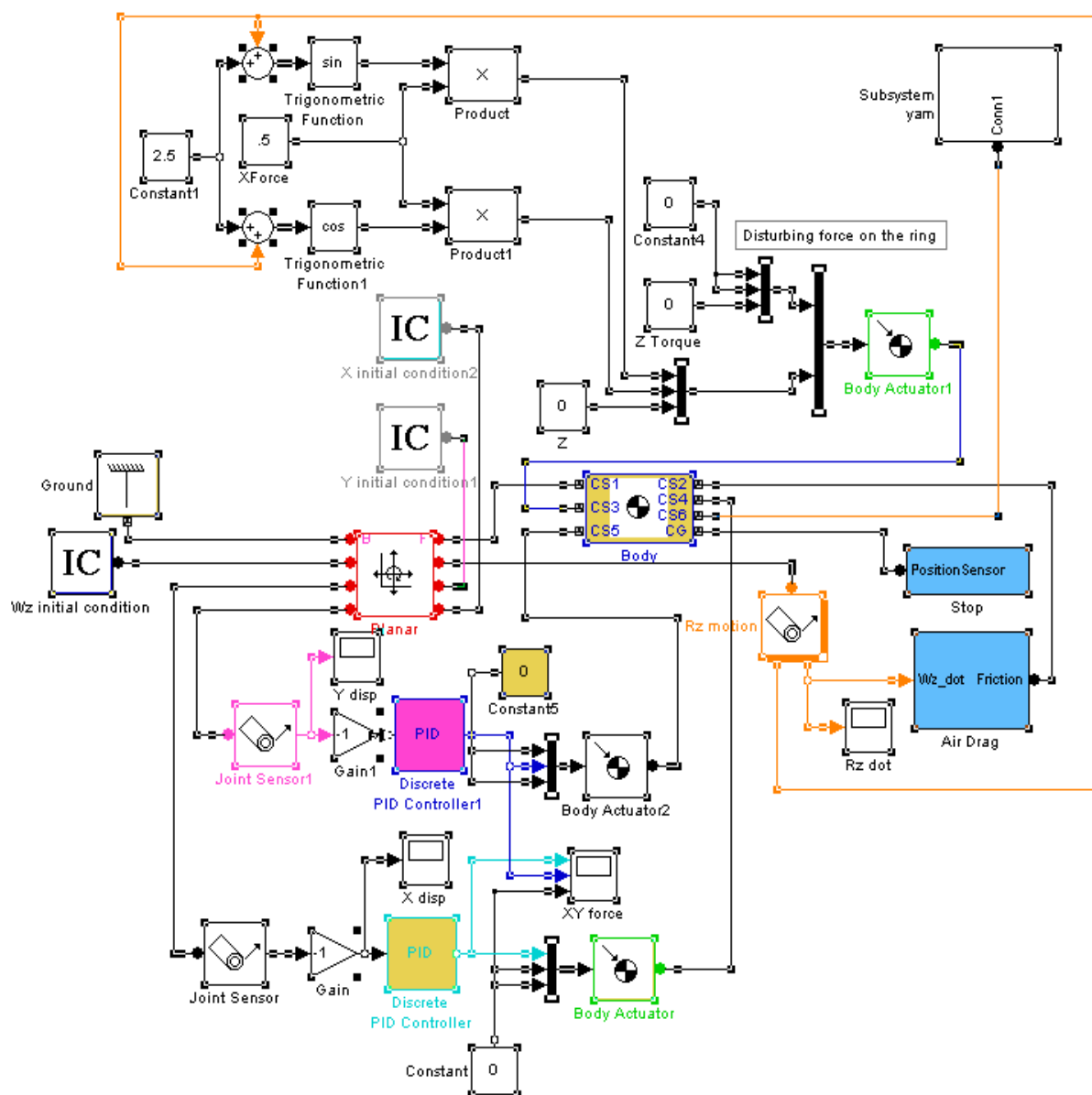
Figure 7. Simulink model
