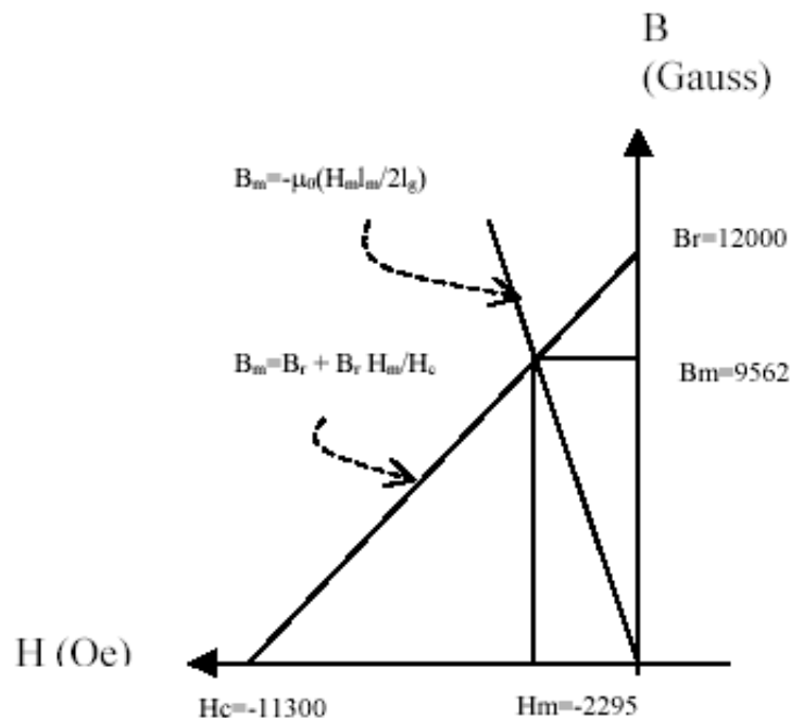
Figure 4. Finding the permanent magnet operating point
