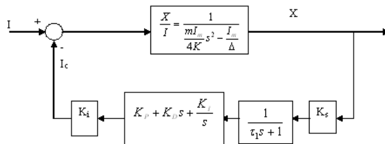
Figure 6. Diagram of the control system
