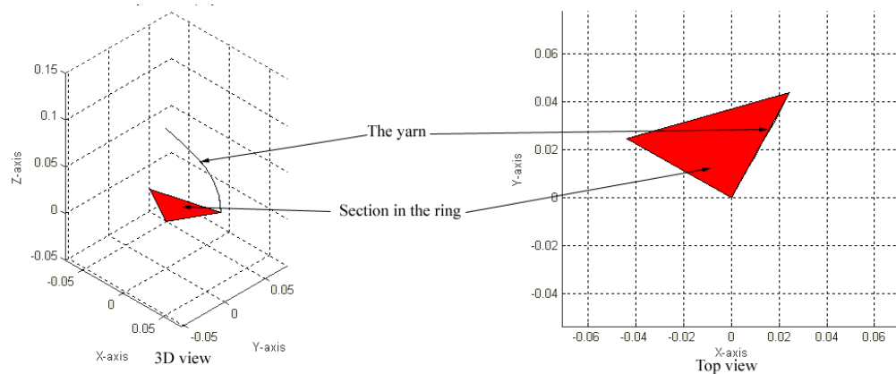
Figure 8b. Yarn balloon at steady state – 3D and top view (700 ms after starting simulation)
