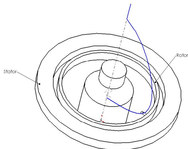
Figure 2. Magnetically suspended rotor in magnetic spinning
