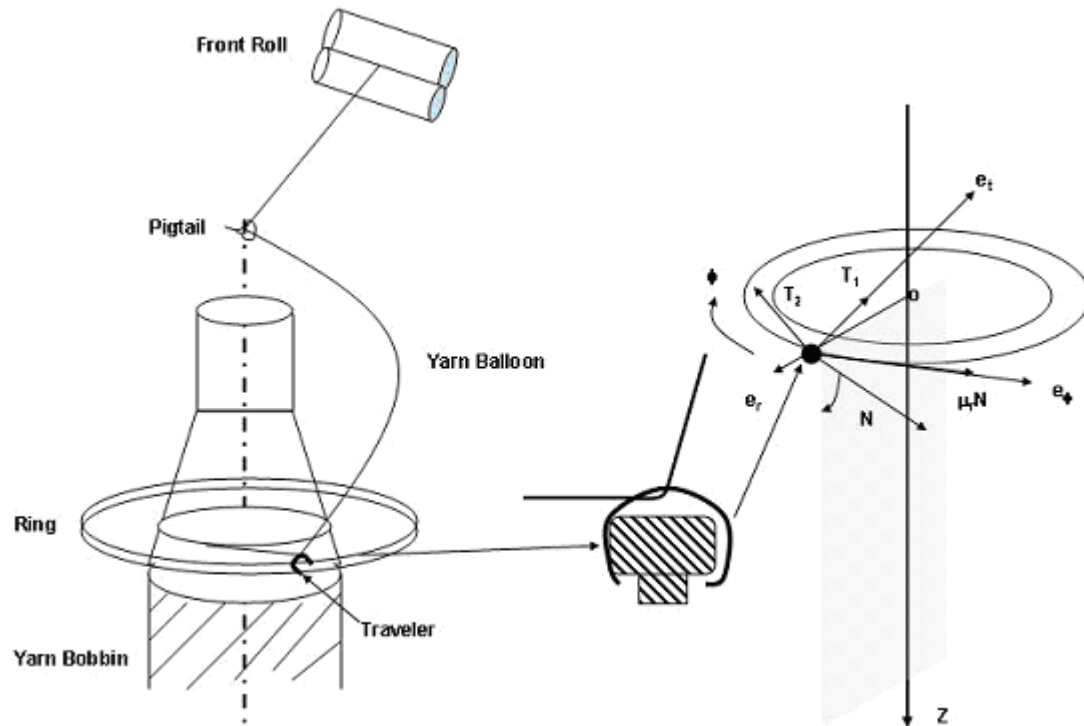
Figure 1. Different forces acting on the traveller [Betra et al, 4]
