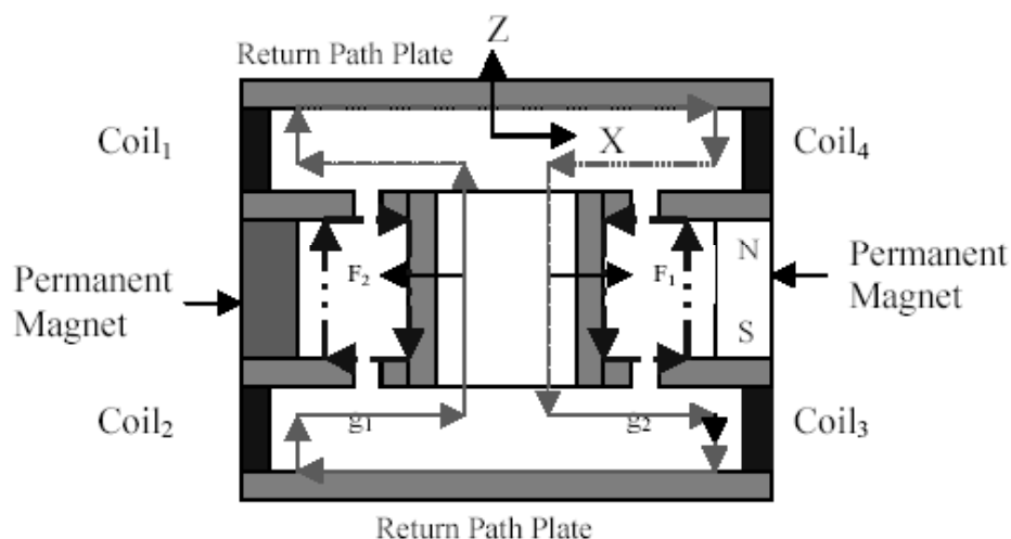
Figure 3. Cross-section of the magnetic system
