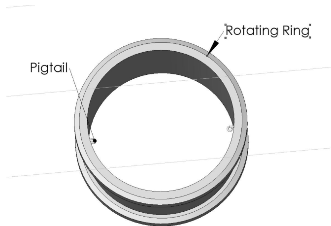
Figure 9. Detail of rotating ring, showing the pigtail for yarn path
