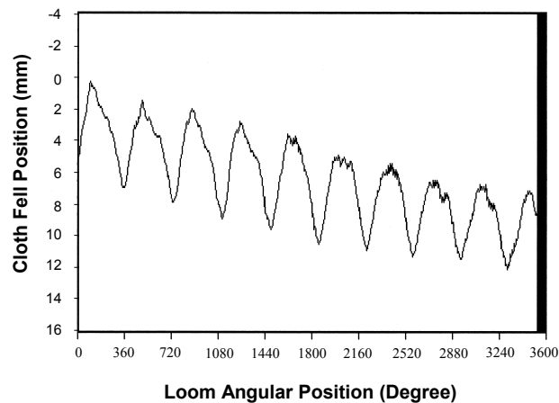
Figure 5. Cloth fell movement dynamic cycle
