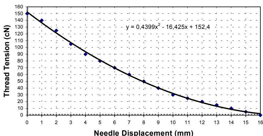
Figure 3. Force-displacement depending calibration curve
