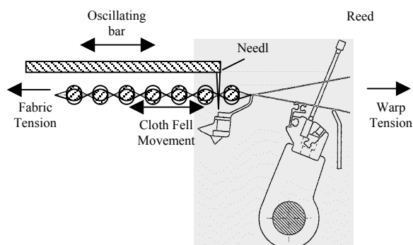
Figure 2. The needle-mechanical device, principal concept
