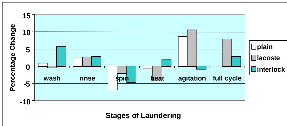
Figure 5: Changes in loop shape factor after five cycles
