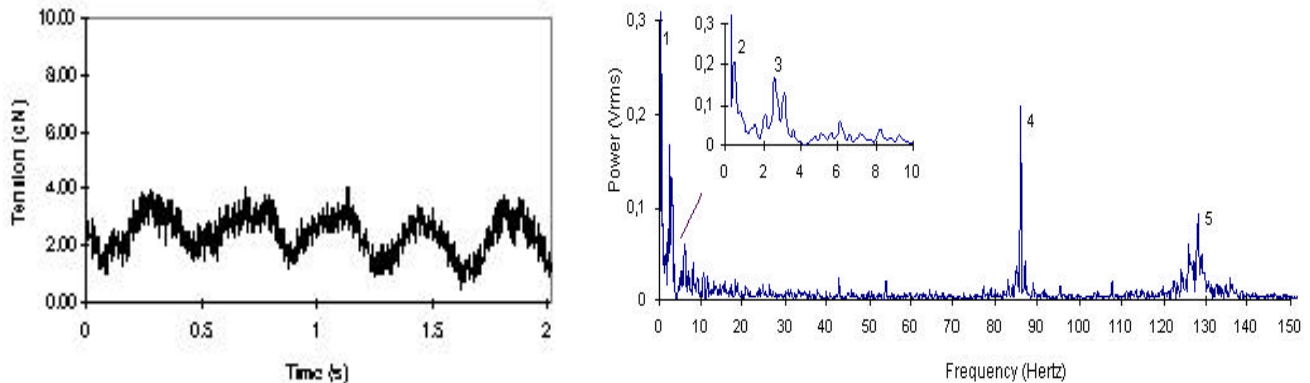
Figure 3. Abnormal feeding system functioning (a) and resulting spectrum (b).
