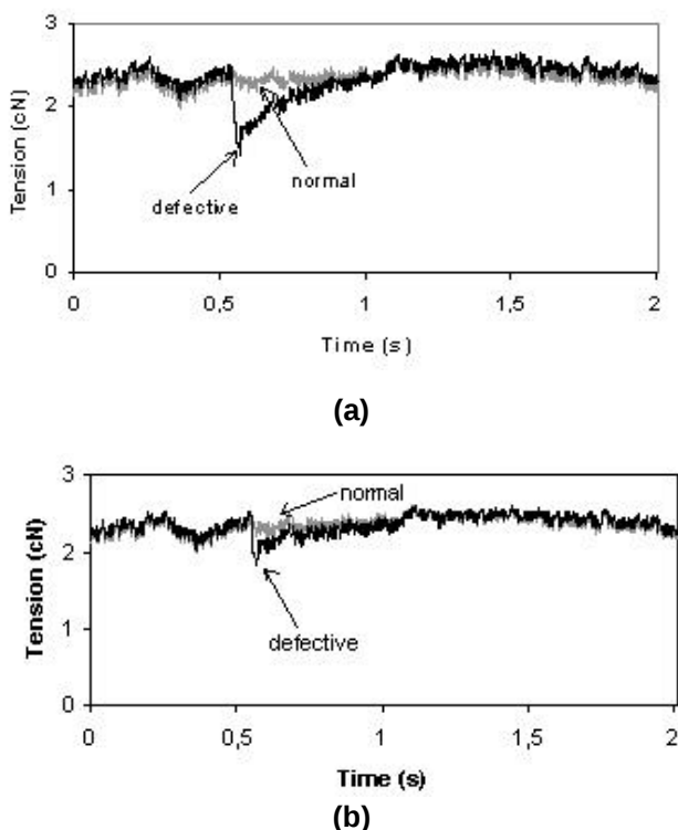
Figure 6. Two examples of defects simulated for polyester 240 dtex yarn: a) needle without hook, and b) no sinker.
