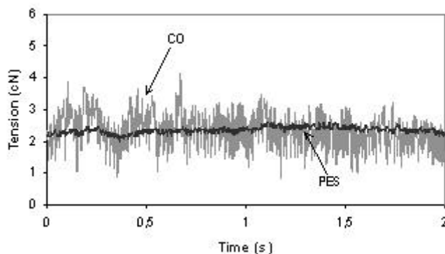
Figure 4. Waveforms for polyester 240 dtex yarn and combed cotton 24 Ne yarn.
