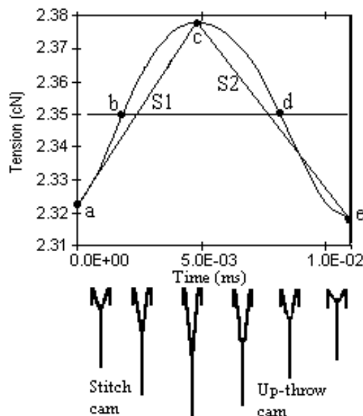
Figure 8. Typical shape of yarn input tension for stitch formation, for polyester yarn.
