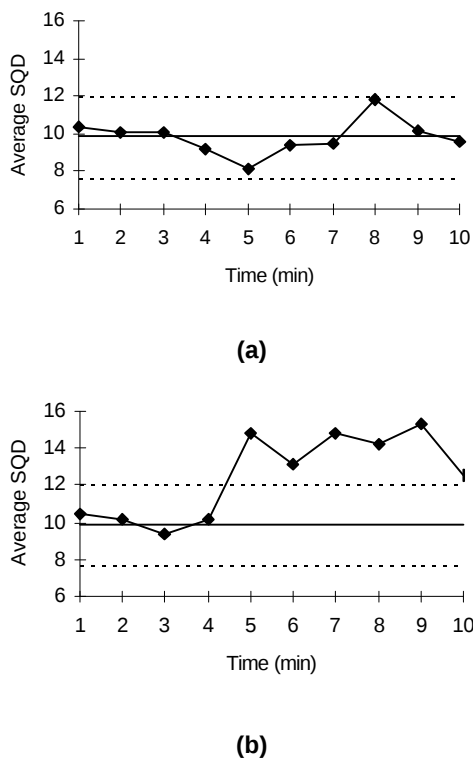
Figure 7. X-chart for knitting production: a) normal functioning; b) a problem with the knitting process.
