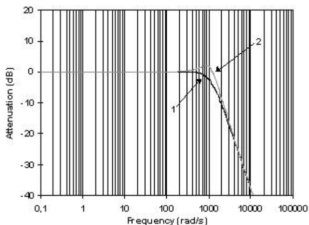
Figure 1. Frequency response of Rothschild tension meter
