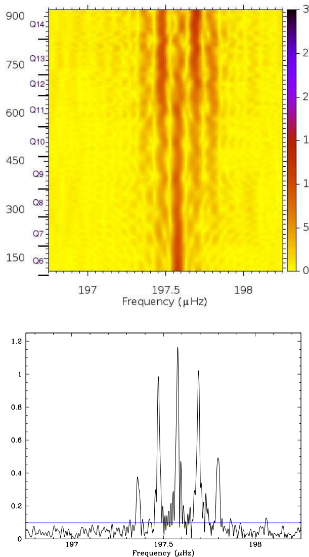
Figure 2. Sliding Fourier transforms (sFTs; top panel) shown with the FT (bottom) of the total data set. Figures from Reed et al. (2014).
