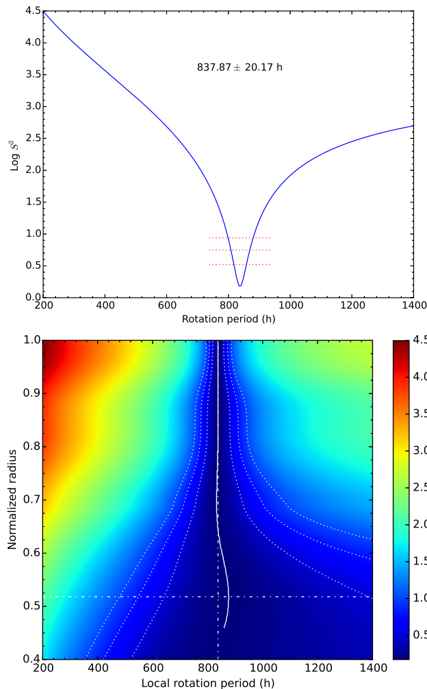
Figure 9. Top panel: Result of the optimization procedure under the hypothesis that PG 1219+534 rotates slowly and rigidly. This shows the behavior of the merit function S^2 in terms of the assumed rotation period. The dotted horizontal lines correspond, from bottom to top, to the 1-, 2-, and 3- \sigma limits. Bottom panel: Result for solid-body rotation using a variable step rotation law. This is a contour map indicating the behavior of the 2D merit function S^2 as a function of depth (expressed in fractional radius) and in terms of the rotation period of the inner region of our two-zone approach. The solution is illustrated by the nearly vertical white curve and the dotted white curves depicting its associated 1-, 2-, and 3- \sigma contours. These contours diverge out at large depths which indicates that the rotationally split p -modes available in the present case lose their capacity to measure the local rotation rate there. The horizontal dot-dashed line indicates the layer above which there is 1% of the mass of the star.
