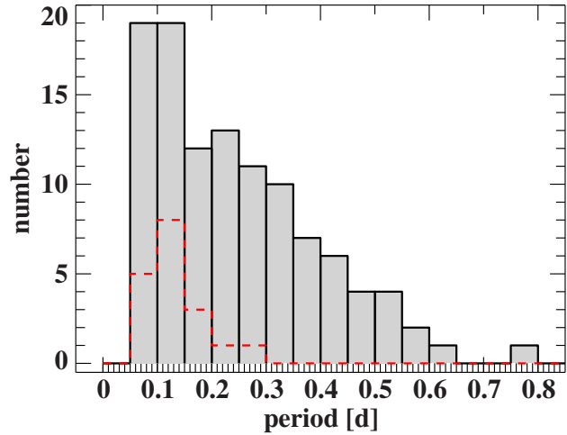
Figure 4. Period distribution of the OGLE HW Vir candidates in comparison to the known HW Vir systems. The OGLE systems are shown in gray and the known systems by the red dashed line.
