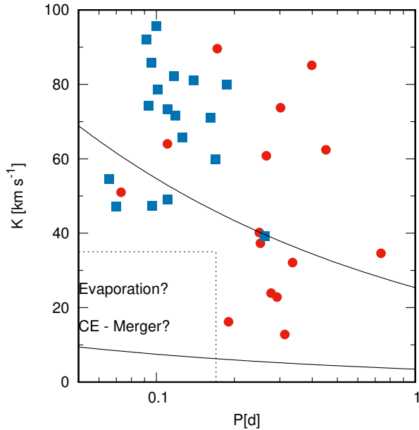
Figure 2. This figure is an updated version of Figure 4 from Schaffenroth et al. (2014a). It shows the RV semi-amplitudes of all known sdB binaries with reflection effects and spectroscopic solutions plotted against their orbital periods. Blue squares mark eclipsing sdB binaries of HW Vir type where the companion mass is well constrained. Red circles mark systems without eclipses, where only lower limits can be derived for the companion masses. The lines mark the regions to the right where the minimum companion masses derived from the binary mass function (assuming 0.47 M_{\odot} for the sdBs) exceed 0.01 M_{\odot} (lower curve) and 0.08 M_{\odot} (upper curve).
