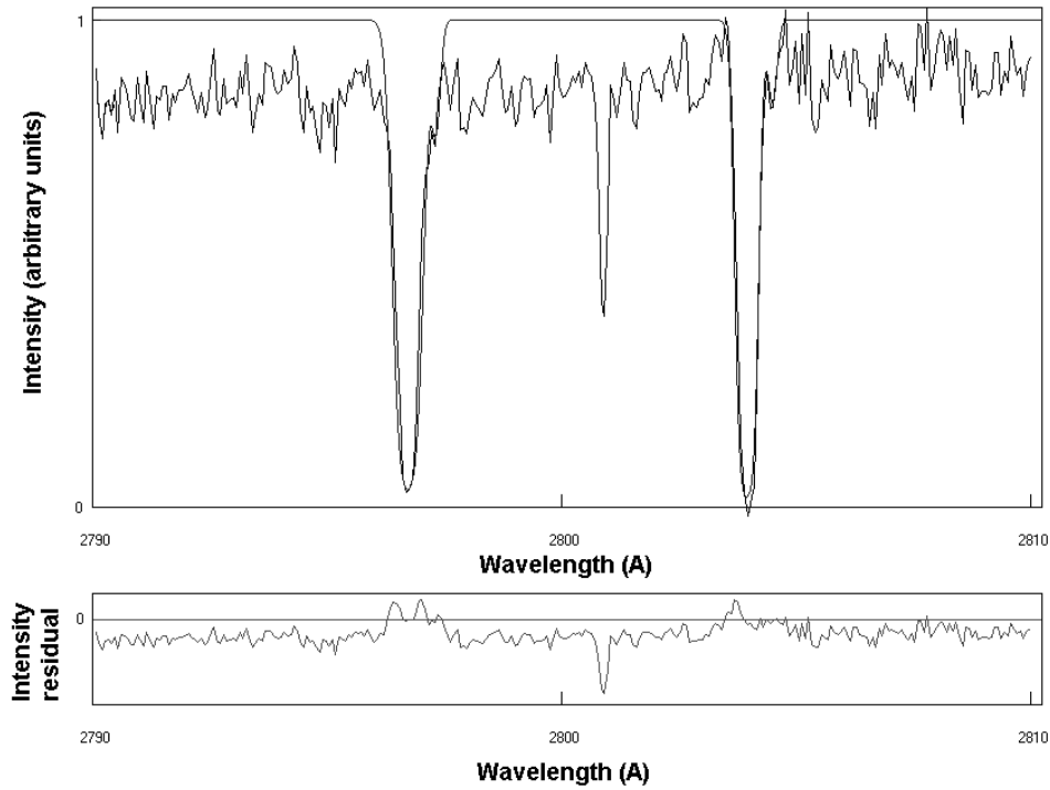
Fig. 1. The UV Mg II resonance lines in the spectrum of HD 52721 with the model fit. The model for each of the Mg II lines consists of two components. The graph at the bottom shows the differences between the model and the observed spectra.
