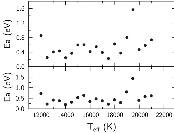
Fig. 4. Absorbed energy of the Mg II lines at \lambda = 2795.523 \text{ \AA} (top) and \lambda = 2802.698 \text{ \AA} (bottom) vs. T_{\text{eff}} .
