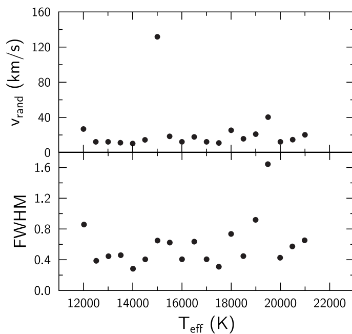
Fig. 3. Random velocities (top) and the FWHM (bottom) of the Mg II resonance lines vs. T_{\text{eff}} .
