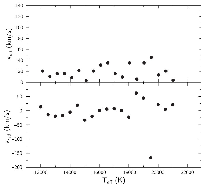
Fig. 2. Rotational (top) and radial (bottom) velocities of all components of the Mg II resonance lines vs. T_{\text{eff}} .
