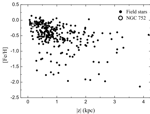
Fig. 7. [\text{Fe}/\text{H}] vs. distance below the Galactic plane for stars in Table 3. NGC 752 is shown as open circle with the error bar representing a standard deviation in [\text{Fe}/\text{H}] (the error bar in distance z is too small to be shown).
