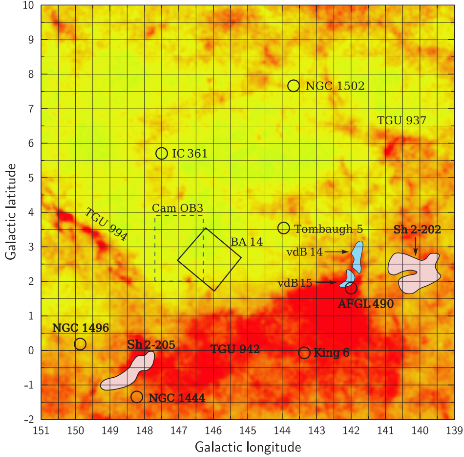
Fig. 1. The position of the Tombaugh 5 cluster with respect to the surrounding objects in the 12^\circ \times 12^\circ area. The chart is based on the Dobashi et al. (2005) atlas of dark clouds (TGU numbers) and shows the positions of the nebulae Sh2-202, Sh2-205, vdB 14 and vdB 15, the open clusters King 6, NGC 1502, IC 361, NGC 1444 and NGC 1496, the association Cam OB3, the dark clouds TGU 937, TGU 942 and TGU 994, and the high-mass YSO AFGL 490. BA 14 is the area investigated by Zdanavičius et al. (2005a,b).
