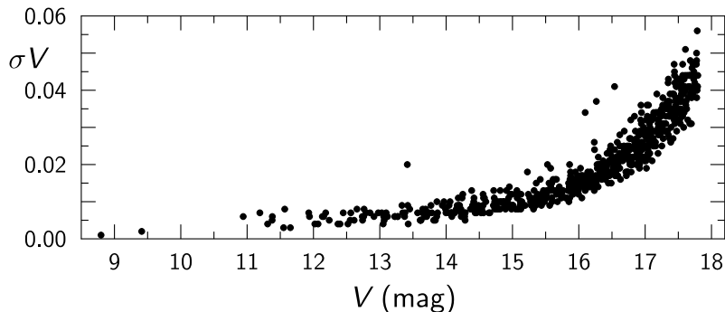
Fig. 4. Single-measurement errors of the magnitude V .
