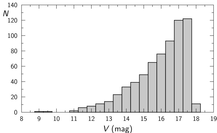
Fig. 3. Star counts in the magnitude V bins.
