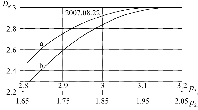
Fig. 1. Plots of the generalized multifractal spectrum D_N(p_{2q}) (a) and D_N(p_{3q}) (b) of small-scale ionospheric turbulence.
