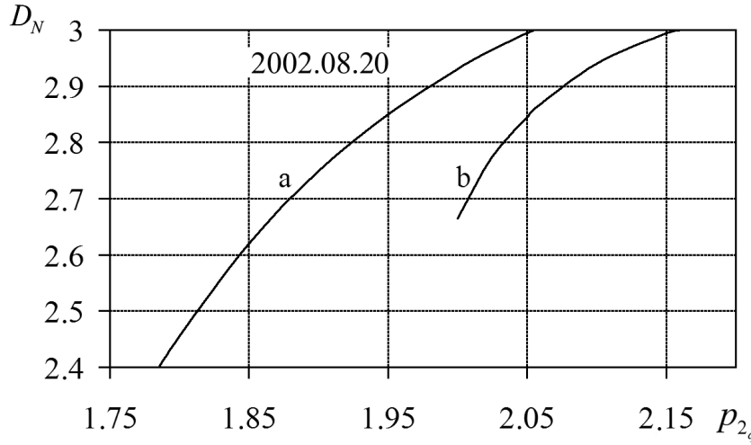
Fig. 2. Plots of the multifractal spectra of small-scale ionospheric turbulence (receiver at the Arya center).
