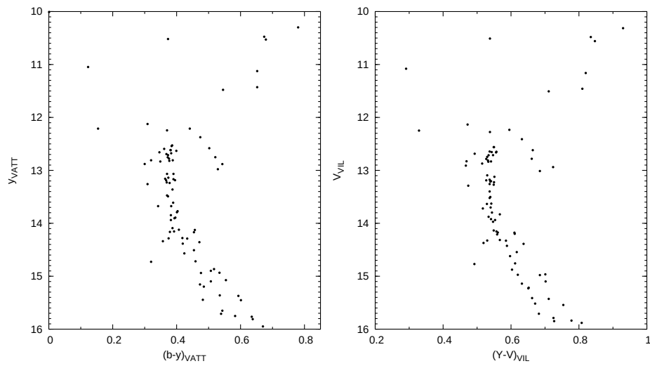
Fig. 1. Comparison of color-magnitude diagrams from VATT and Laugalys et al. (2003) in the Vilnius system. Only common stars are plotted.
