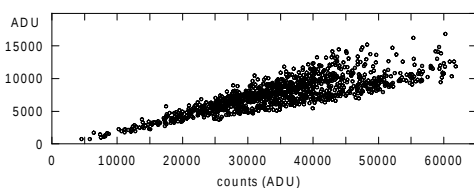
Fig. 2. Maximum count rates for \eta Car (X-axis) and HD 303308 (Y-axis). Source: Sterken et al. (2001).
