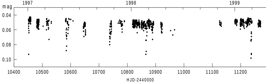
Fig. 6. y magnitude differences between 13''.3 and the 23''.0 apertures (Sterken et al. 2001).
