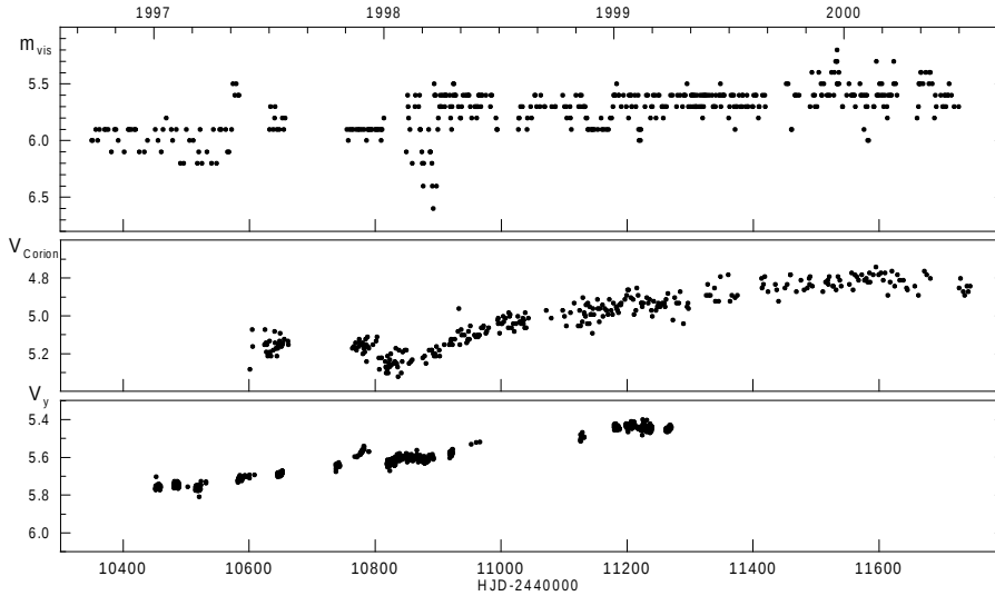
Fig. 4. Top: visual magnitude estimates of \eta Car, middle: CCD photometry with Corion NR-400 V filter, bottom: y -CCD photometry ( 23''.0 aperture). Source: Sterken et al. (2001).
