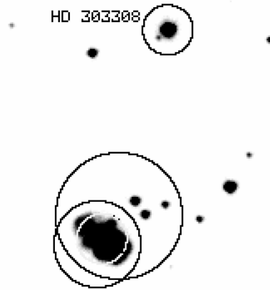
Fig. 5. Field of \eta Car with calibration star HD 303308 (see text).
