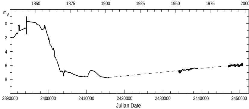
Fig. 1. Visual light curve of \eta Car since the primary eruption (Sterken 2003).
