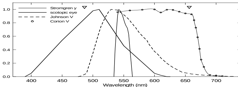
Fig. 3. y , V and Corion normalized transmissions. \nabla : H\beta and H\alpha .
