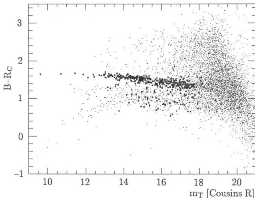
Fig. 14. Color-magnitude relation for the central 75 \text{ arcmin} \times 80 \text{ arcmin} of the Coma cluster. Both stars and galaxies are included on this figure, a total of 15 370 objects. The lack of objects in the upper right hand corner is due to the combination of the magnitude limits in B and R_c . Small black points – stars; black boxes – spirals and irregulars, confirmed members; dark grey boxes – E and S0 galaxies, confirmed members; light grey boxes – unclassified confirmed members; small grey points – other galaxies in the field, members and non-members. The photometric data are from Jørgensen (2000). The redshift data are from Jørgensen & Hill (2000).
