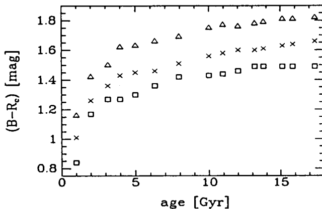
Fig. 13. Example of the predictions from the Vazdekis et al. (1996) models: (B-R_c) color as function of age (the x -axis) and metallicity (the different symbols). Triangles – [M/H] = 0.4 ; crosses – [M/H] = 0.0 ; boxes – [M/H] = -0.4 . It is seen that the stellar populations get redder with higher age and higher metallicity.
