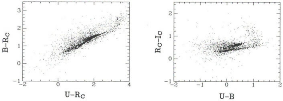
Fig. 15. Optical color-color relations for the Coma cluster. Symbols as in Fig. 14. Solid line on the left panel – SPP models from Vazdekis et al. (1996), see text.
