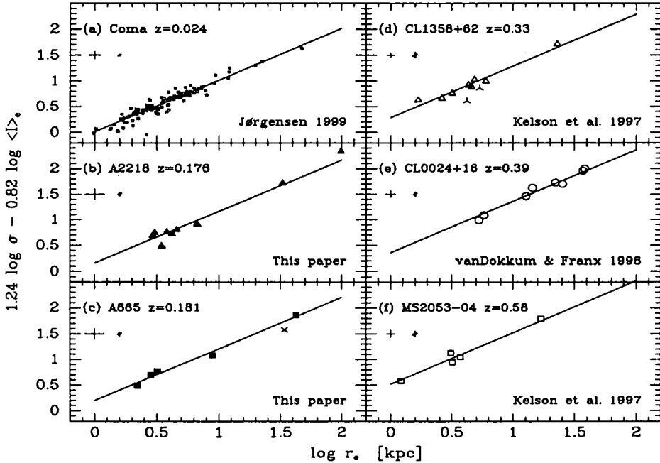
Fig. 18. The FP edge-on for Coma, A 2218, A 665, CL 1358+62, CL 0024+16 and MS 2053-04. The sources of the data are given on the panels ('This paper' refers to Jørgensen et al. 1999). The skeletal symbols on panels (c) and (d) are the E+A galaxies. The photometry is calibrated to Gunn r in the rest frames of the clusters. The mean surface brightness \log \langle I \rangle_e = -0.4(\langle \mu \rangle_e - 26.4) is in units of L_\odot/\text{pc}^2 (cf. Section 2.4.1). The photometry is not corrected for the dimming due to the expansion of the Universe. The effective radii are in kpc ( H_0 = 50 \text{ km}/(\text{s Mpc}) and q_0 = 0.5 ). The solid lines are the FPs with coefficients adopted from Jørgensen et al. (1996) and with zero points derived from the data presented in the figure. Typical error bars are given on the panels; the thin and thick error bars show the random and systematic uncertainties, respectively. (From Jørgensen et al. 1999.)
