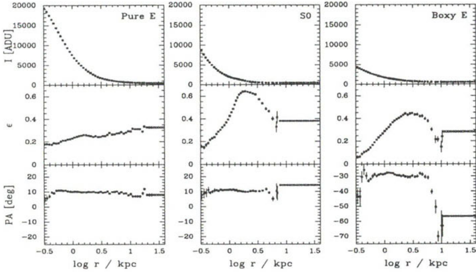
Fig. 4. Radial profiles of intensity, ellipticity and position angle for the three example galaxies. The plotted range in equivalent radii r is 0.3–40 kpc (0.8–102 arcsec).
