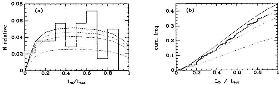
Fig. 12. Relative (a) and cumulative (b) frequency for the relative disk luminosities. Solid line – determinations from the \epsilon_{21.85}-\langle c_4 \rangle diagram. The distribution has been normalized with the total number of galaxies fainter than m_T = 12^m7 . Dashed line – model prediction for a uniform intrinsic distribution, corrected for the incompleteness due to the limits enforced on \epsilon_{21.85} and \langle c_4 \rangle . Dotted lines – model predictions for a uniform intrinsic distribution plus a fraction of diskless galaxies. Models for fractions of 0.1, 0.2, and 0.5 are shown. A higher fraction of diskless galaxies moves the curve for the normalized distribution downwards in both (a) and (b). (From JF94).
