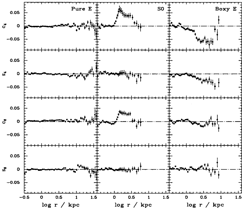
Fig. 8. Radial profiles of the Fourier coefficients c_4 , s_4 , c_6 and s_6 for the three example galaxies. The plotted range in equivalent radii r is 0.3–40 kpc (0.8–102 arcsec). Points with uncertainty larger than 0.025 are not plotted.
