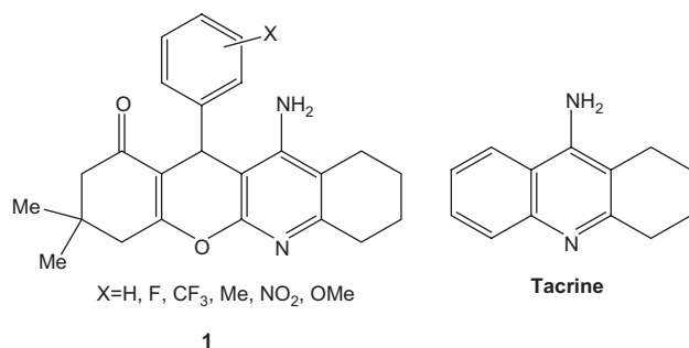
Figure 1 Structure of compound 1 and tacrine.
