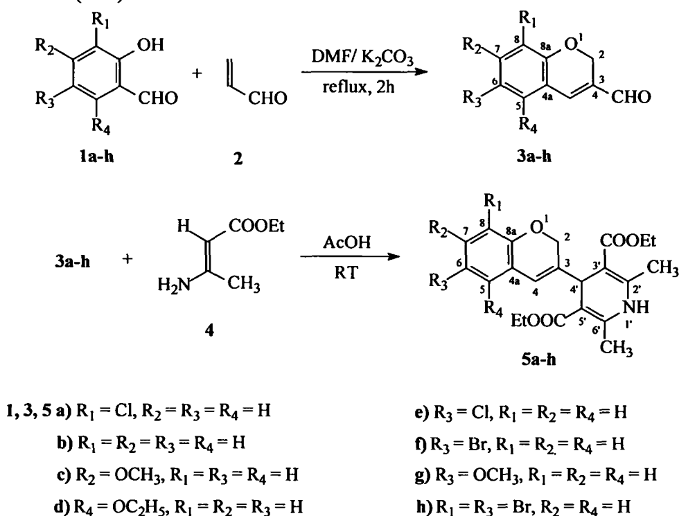
Scheme-1: Synthesis of 3-[4'-(2',6'-dimethyl-3',5'-dicarbethoxy-1',4'-dihydropyridyl)]chromenes ( 5a-h )
