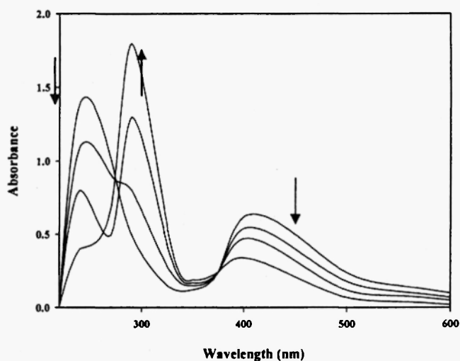
Fig. 4 Absorption spectra of 10^{-3} M bromine in the presence of varying quantities of TT12C4 in \text{CHCl}_3 solution. The [TT12C4]/[Br 2 ] mole ratios are: 0.0, 0.5, 1.0, 1.5.
