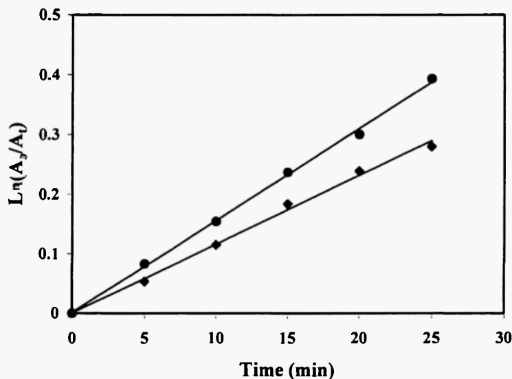
Fig. 12 Plots of \text{Ln}(A_0/A_t) vs. time for 10^{-3} M of bromine and 10^{-3} M of HT18C6 in \text{CH}_2\text{Cl}_2 (●) and \text{CHCl}_3 (◆) solutions.
