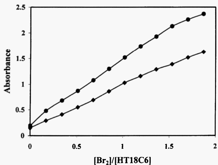
Fig. 7 Plots of absorbance vs. [\text{Br}_2]/[\text{HT18C6}] in \text{CH}_2\text{Cl}_2 (●) and \text{CHCl}_3 (◆) solutions.
