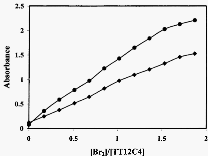
Fig. 6 Plots of absorbance vs. [\text{Br}_2]/[\text{TT12C4}] in \text{CH}_2\text{Cl}_2 (●) and \text{CHCl}_3 (◆) solutions.
