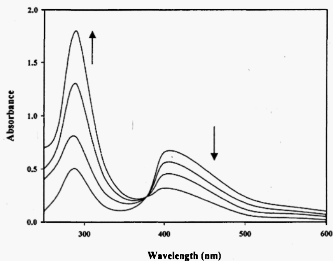
Fig. 5 Absorption spectra of bromine in the presence of varying quantities of HT18C6 in \text{CHCl}_3 solution. The [HT18C6]/[Br 2 ] mole ratios are: 0.0, 0.5, 1.0, 1.5.
