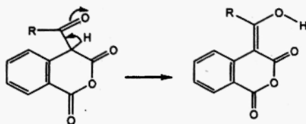
Scheme 2 : Mechanism of formation of 4-Acyl isochroman-1,3-diones.
