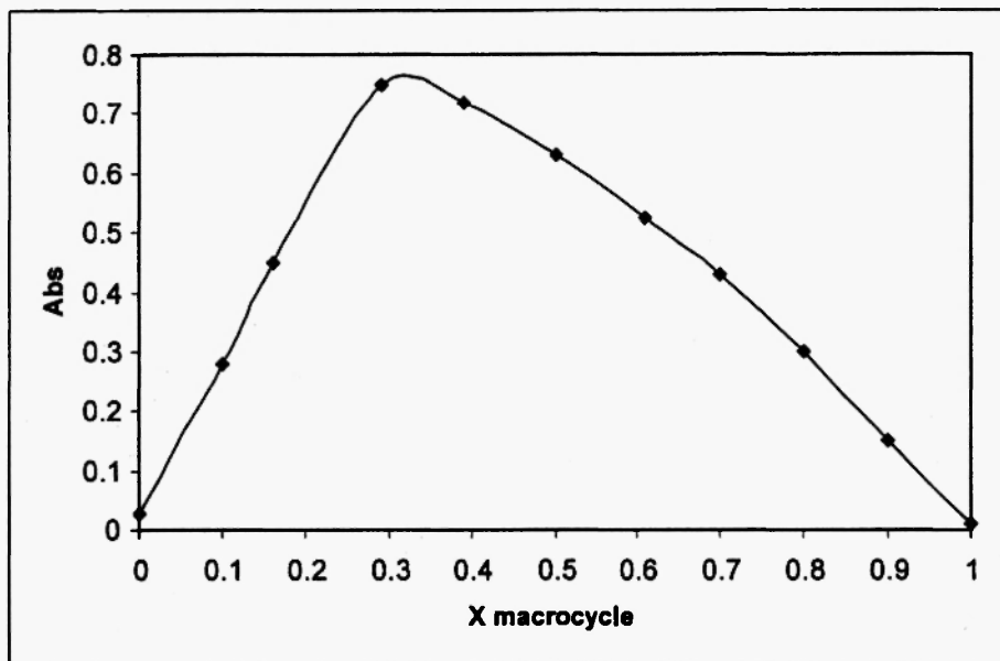
Figure-3 : Continuous variation plot for TMTA14C4-IBr at \lambda = 360 nm.
