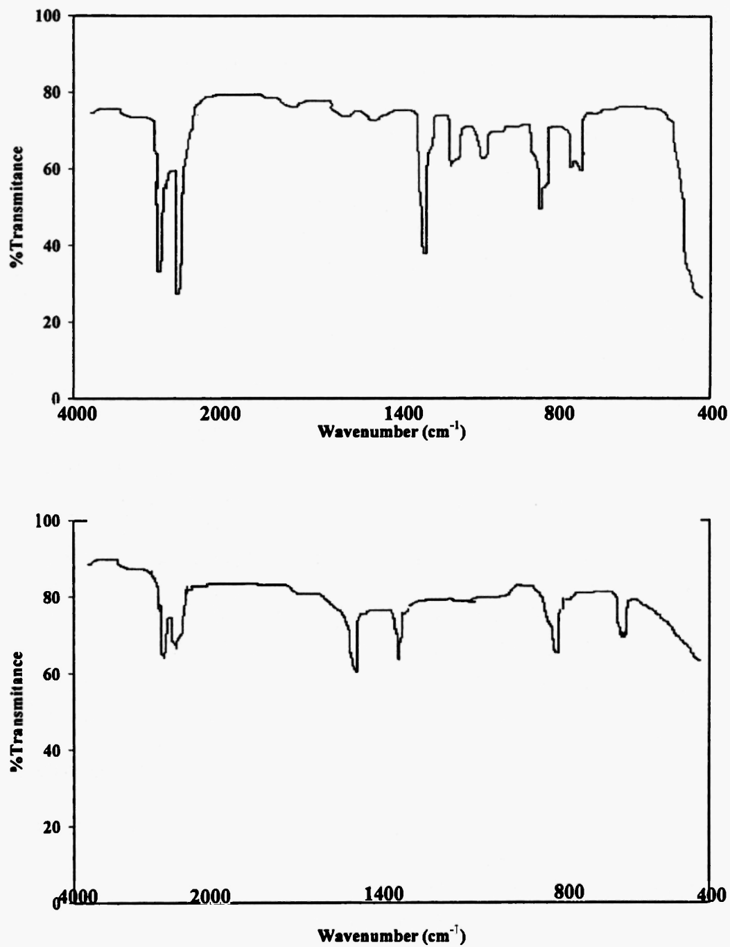
Figure-6 : IR spectra of TMTA14C4 (up) and TMTA14C4-IBr complex (down).
