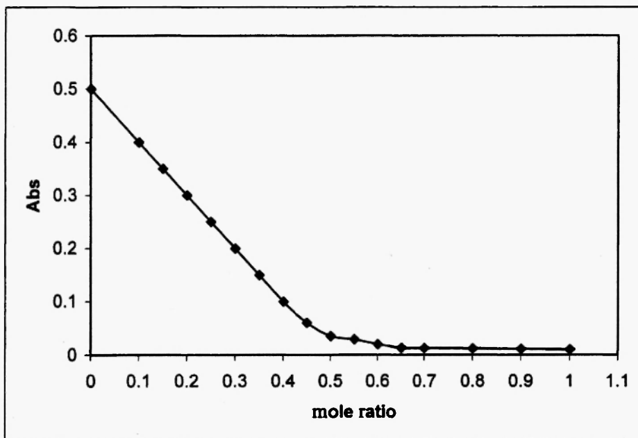
Figure-2 : Plot of absorbance vs. TMTA14C4/IBr at \lambda = 508 nm.
