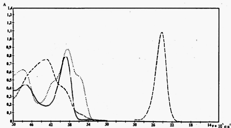
Figure-2 : UV-VIS spectrum of a) keto form (—), b) enol form (---) barbituric acid immediately after solvating in water c) enol form after 5 days from moment solvating in water (···)
