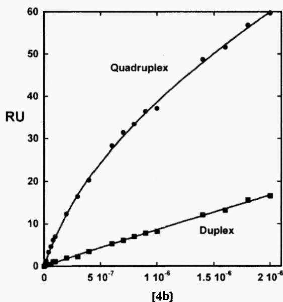
Figure-1: Sensorgrams for the interaction of 4b with the 5'-biotin-labeled HuTelo and AATT duplex were collected in 0.1 M KCl, 0.01 M Tris, 0.003 M EDTA, pH 7.3 over a 4b concentration range from 10 nM to 2.0 \mu M (flow rate of 40 \mu L/min at 25°C). The response (RU) in the plateau region of the sensorgrams at each 4b concentration were determined and binding isotherms for 4b complexes with the HuTelo and AATT were obtained by plotting RU versus the compound concentration. The lines in the Figures were obtained by non-linear least-squares fits of the data to one and two site binding equations as described in the Methods Section.
