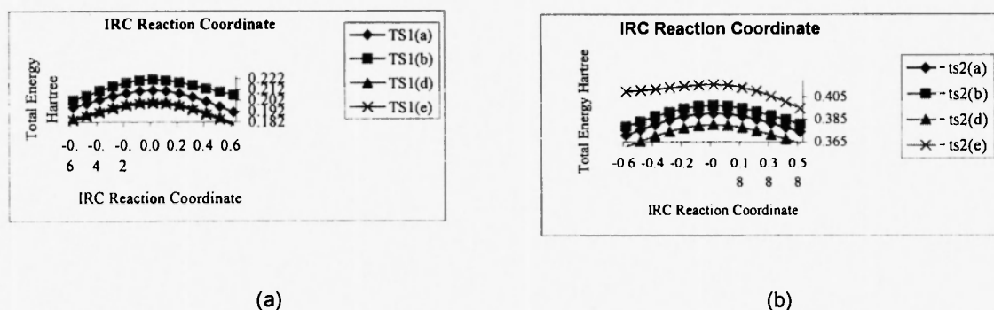
Figur-4 : IRC Reaction Coordinates of TS1 and TS2 for 5(a), 5(b), 5(d) and 5(e) products
