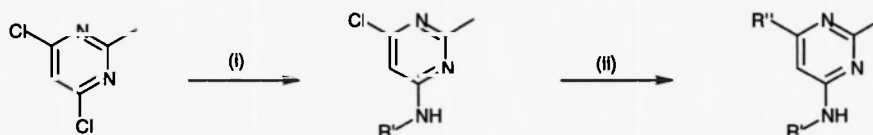
Scheme 3. Reagents and Conditions: (i) R'_2NH , 5M LPDE, rt, 16h; (ii); R''_2NH , sealed tube, 160°C, 24 h.
