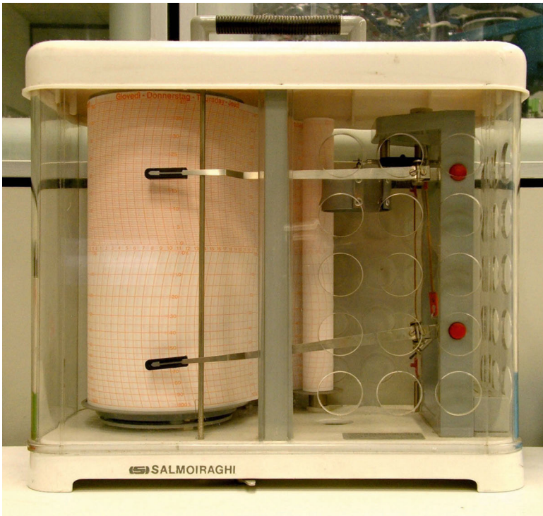
Abb. 2: Hygrograph
