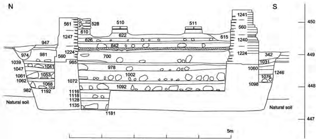
Fig. 4.33: West-facing composite section across the South Temple showing foundations.
