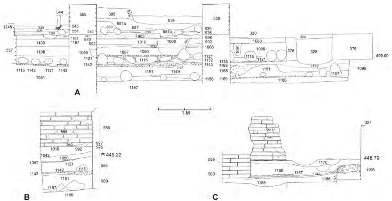
Fig. 4.22: Test Pit 9 sections. (A) Composite section across the whole test pit and the mandapa of the North Temple looking west. (B) East-west section against wall 556 below the southern part of wall 558 where it crosses the test pit. (C) The western section of the test pit to the north of the Phase I structure showing the edge of foundation cut 1171.
