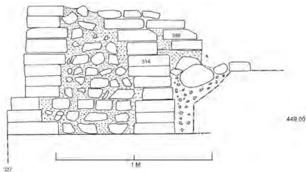
Fig. 4.19: East-west section through wall 514 showing extra face 559/1213.
