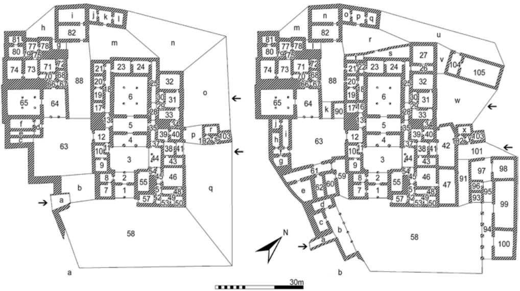
Figure 2 | Pylos, palace: a) plan of earlier building state with room numbers, points of access indicated by arrows; b) plan of later building state with room numbers, points of access indicated by arrows.
