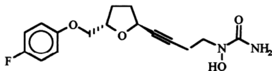
Scheme 1 CMI-977 (I). (2 S ,5 S )- trans -5-(4-Fluorophenoxymethyl)-2-(1- N -hydroxy-ureidyl-3-butyn-4-yl)-tetrahydrofuran.
