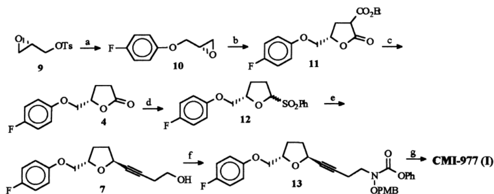
Scheme 3 Reagents: (a) 4-Fluorophenol, \text{NaH} , (b) \text{CH}_2(\text{CO}_2\text{Et})_2, \text{Na} , (c) DMA, \text{MgCl}_2 \cdot 6\text{H}_2\text{O} , (d) (i) DIBAL (ii) \text{PhSO}_3\text{H} , \text{CaCl}_2 , (e) (i) i\text{PrMgBr} , \text{HC}\equiv\text{C}(\text{CH}_2)_2\text{OTHP} , \text{ZnBr}_2 (ii) 1% \text{HCl} (iii) crystallizations, (f) \text{PhOCONHOPMB} , \text{Ph}_3\text{P} , DEAD, (g) (i) \text{NH}_3 (ii) \text{BF}_3 \cdot \text{OEt}_2 .
