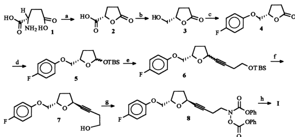
Scheme 2 Reagents: (a) \text{HNO}_2 , (b) \text{BH}_3 \cdot \text{Me}_2\text{S} , (c) 4-Fluorophenol, \text{Ph}_3\text{P} , DIAD, (d) (i) DIBAL (ii) TBSCl, Imid., DMAP, (e) (i) TMSBr (ii) n\text{-BuLi} , \text{HC}\equiv\text{C}(\text{CH}_2)_2\text{OTBS} , (f) (i) TBAF (ii) separation of trans from trans/cis isomers by crystallization (g) \text{PhOCONHOCOOPh} , \text{Ph}_3\text{P} , DIAD, (h) \text{NH}_4\text{OH} .
