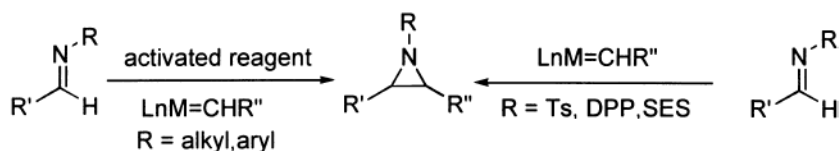
Scheme 11
