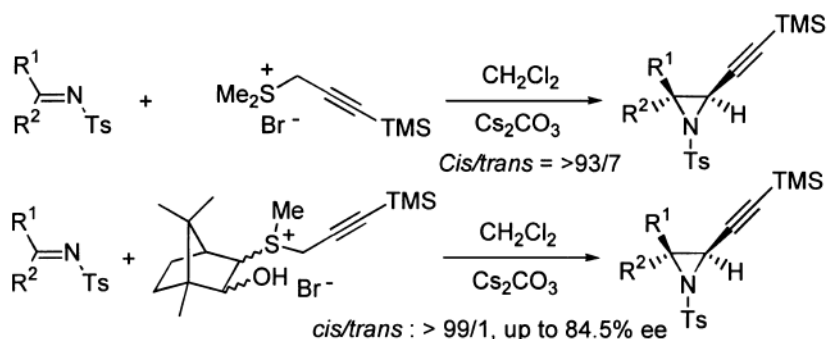
Scheme 13
