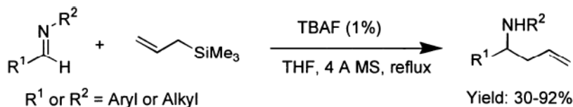
Scheme 8
