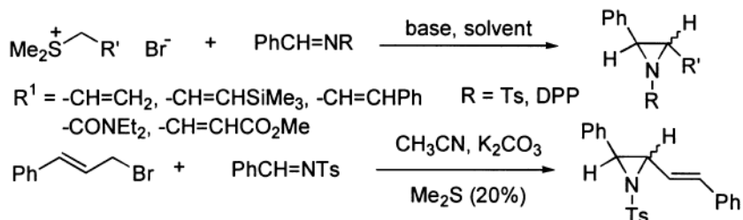
Scheme 12
