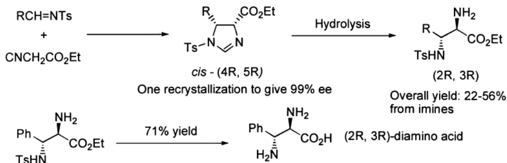
Scheme 4
