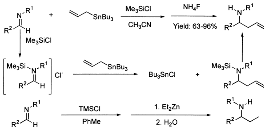
Scheme 6
