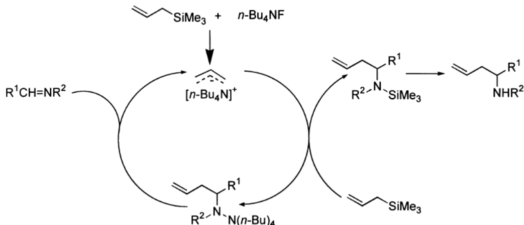
Scheme 10
