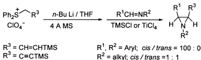
Scheme 14
