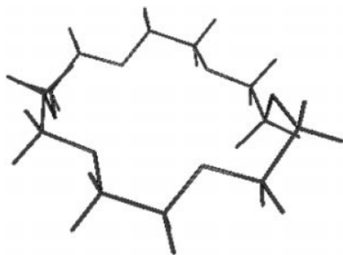
Fig. 5 A Dreiding-stick model of 18-crown-6.
