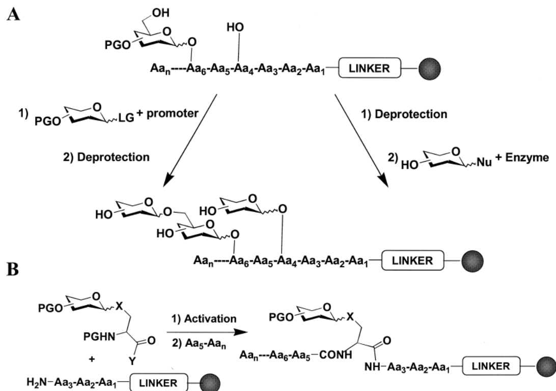
Fig. 2 Strategies for glycopeptide synthesis. (A) Chemical or enzymatic glycosylation of peptide or glycopeptide; Nu = nucleotide sugar. (B) The building block approach ( X = O, C, S, N ; Y = suitable leaving group).
