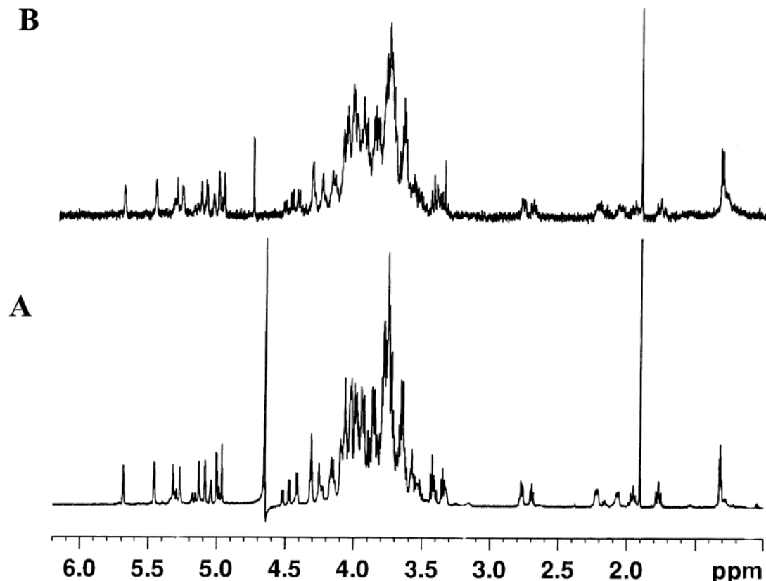
Fig. 1 (A) 750 MHz NMR spectrum, 32 scan at 37 °C, of an 22-mer oligosaccharide, 2.0 mg in 600 µL, from Salmonella enterica ssp. Typhimurium 1135 LPS. (B) NMR spectrum of the same compound 0.14 mg in 40 µL in a nanoprobe operating at 500 MHz, 32 scan at 25 °C.
