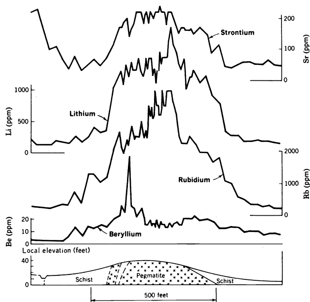
Fig.1 Geochemical soil anomalies related to the underlying bedrock. Note beryllium anomaly indicating location of a beryl-rich zone in the pegmatite. (Hawkes & Webb, 1962)
