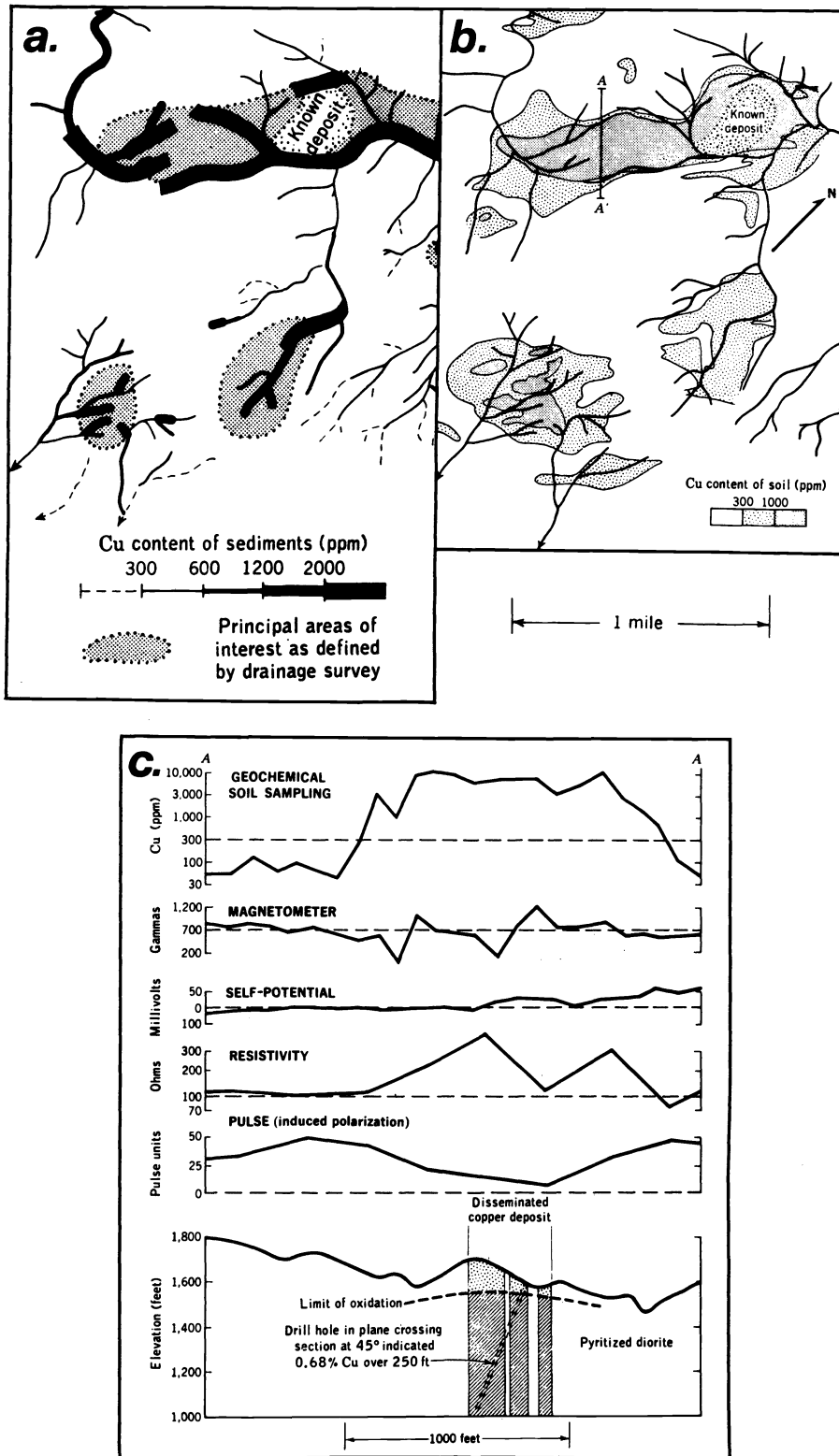
Fig.2 A typical case history illustrating phased exploration: (a) stream sediment reconnaissance to delineate possible areas of interest, (b) follow-up soil survey leading to (c) drilling of the target defined by multi-source data (Hawkes & Webb, 1962)
