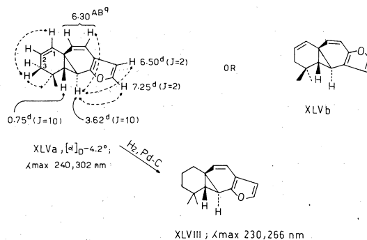
Fig. 17. Structure of spiniferin-1; Chemical shifts in ppm from TMS ( CCl_4 ); coupling constants in Hz; ---- long range proton interaction detected by decoupling.
