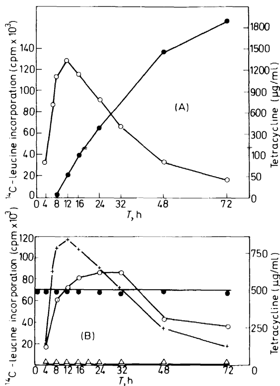
Figure 9. (A) Incorporation of ^{14}\text{C} -leucine into proteins of tetracycline-producing strain of Streptomyces aureofaciens (○—○) and production of tetracycline (●—●). (B) Effect of tetracycline on incorporation of ^{14}\text{C} -leucine into proteins. Course of ^{14}\text{C} -leucine incorporation after addition of tetracycline to 4h cultures: 50\ \mu\text{g ml}^{-1} (+—+); 500\ \mu\text{g ml}^{-1} (○—○) and 1000\ \mu\text{g ml}^{-1} (△—△). In the experiment with 500\ \mu\text{g TC ml}^{-1} the level of tetracycline was followed during the experiment (●—●)
