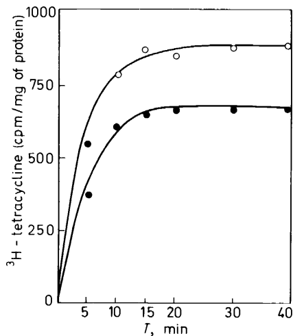
Figure 11. Uptake of ^3\text{H} -tetracycline by tetracycline-producing (●—●) and non-producing (O—O) strains of Streptomyces aureofaciens . The 4h-old cells were incubated at 30^\circ\text{C} with 500\ \mu\text{g ml}^{-1} of ^3\text{H} -tetracycline ( 10\ \mu\text{Ci} ). The samples were suspended in 10\text{mM} Tris-HCl buffer at pH 7.5 and filtered through a membrane filter. Radioactivity of washed cells was counted in a Bray's solution
