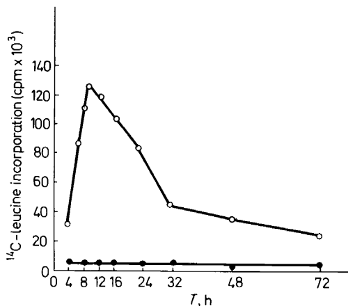
Figure 10. Incorporation of ^{14}\text{C} -leucine into proteins of a tetracycline-nonproducing strain of Streptomyces aureofaciens . ^{14}\text{C} -leucine incorporation in absence (O—O) and presence of 500\ \mu\text{g ml}^{-1} tetracycline (●—●)
