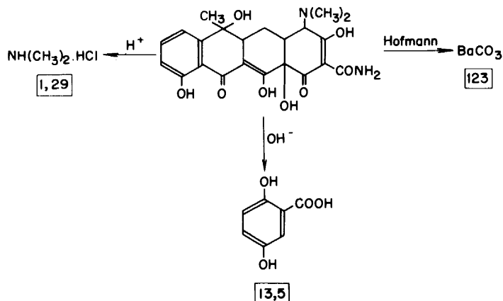
Figure 7. Scheme of tetracycline degradation and the values of the radioactivity (r.m.a. \times 10^{-3}/1C )
