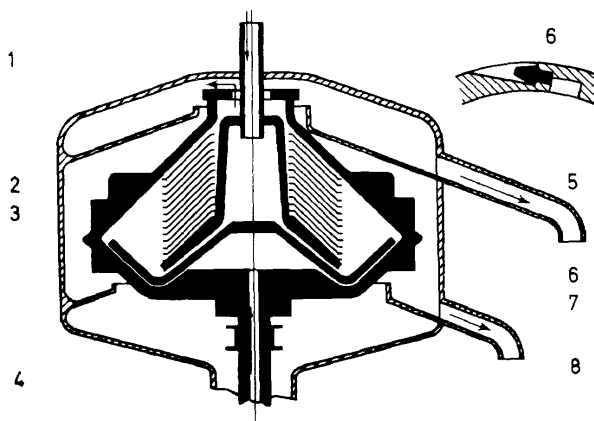
Figure 3. Disk separator
