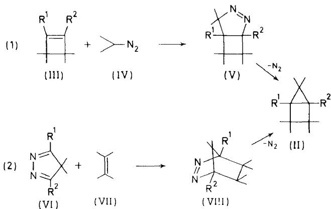
Scheme I. Synthetic approaches to bicyclo[2.1.0]pentane
