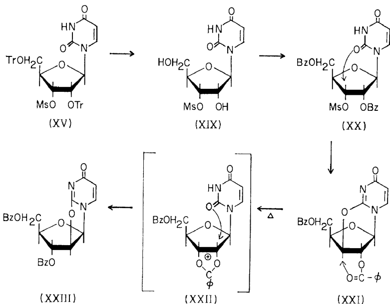
Figure 9. Rearrangement of a 2,3'-anhydronucleoside to a 2,2'-isomer via an orthoester ion 14 zoylated to 3',5'-di-O-benzoyl-3'-O-mesyluridine (XX). Treatment of XX with sodium benzoate in DMF gave the 2,3'-anhydro-xylo-nucleoside (XXI). (Compound XXI was also obtained by direct benzylation of 2,3'-anhydro-xylosyluracil). When XXI was heated in a melting point tube, it melted and resolidified. The resolidified product was the 2,2'-anhydro-arabino-nucleoside (XXIII). Thus, in one step, anhydro bond and benzoyl migration occurred. A most plausible mechanism for this rearrangement is obviously neighbouring group participation by attack of the 2'-benzoate of XXI on C-3' to give a transient orthoester ion (XXII) which then undergoes attack by the 2-carbonyl on C-2' to give the 2,2'-anhydro-arabino nucleoside (XXIII).
