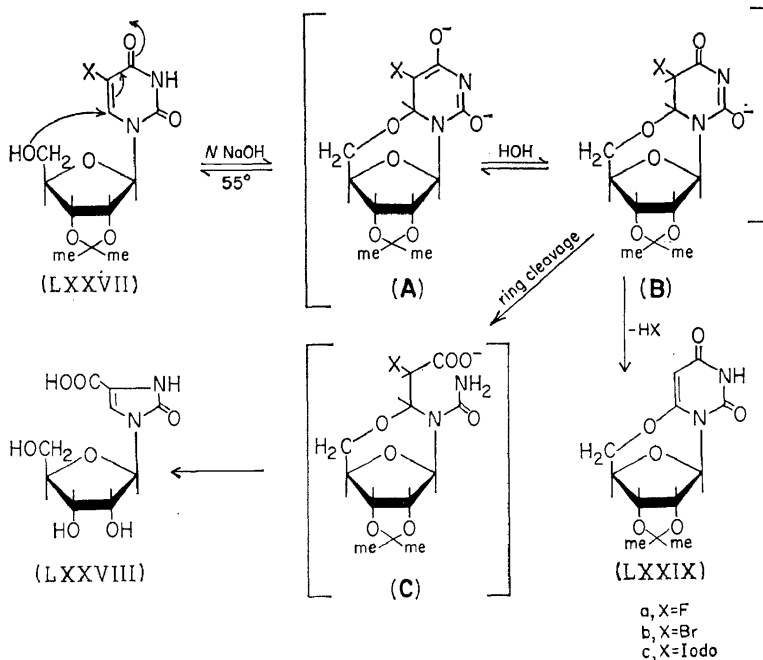
Figure 25. Conversions of 5-halogenated-2',3'-O-isopropylideneuridines to 1- \beta -D-ribofuranosyl-2-oxo-4-imidazoline-4-carboxylic acid and/or the acetone of 6,5'-anhydro-1-( \beta -D-ribofuranosyl)-barbituric acid. 37a,b
