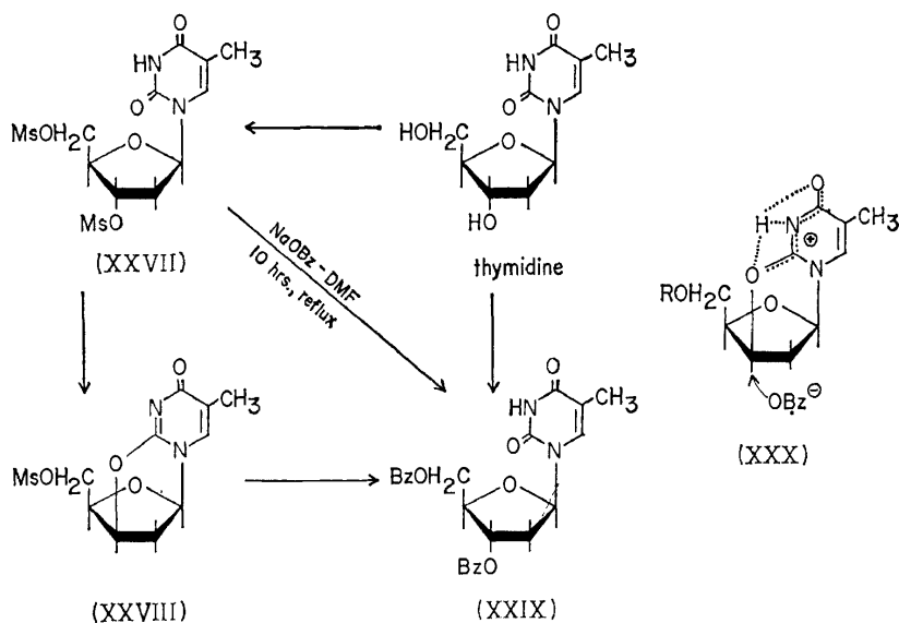
Figure 11. Reactions of 3',5'-di-O-mesylthymidine 16
